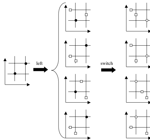
Figure 5: The same effect with left followed by switch
