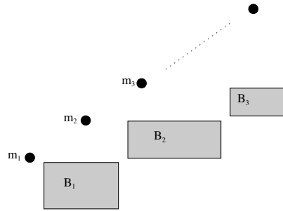
Figure 2: Structure of a permutation in av(2431, \mathcal{IW})
