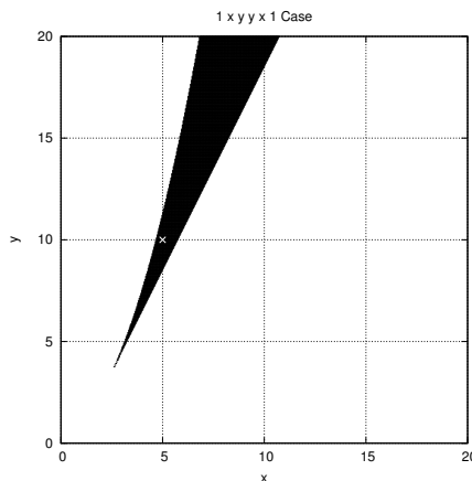
Figure 1: The filled region is the numerical region of \infty -logconcavity for the 2-D even case. The X indicates the position of the binomial coefficient.
