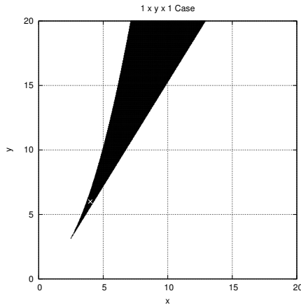
Figure 2: The filled region is the numerical region of \infty -logconcavity for the 2-D odd case. The X indicates the position of the binomial coefficient.
