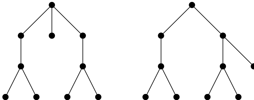
Figure 3: Two trees with degree sequence (2, 2, 3, 3, 3, 1, 1, 1, 1, 1) . The tree on the l.h.s. has smallest maximum eigenvalue ( \lambda = 2.1010 ) among all trees in \mathcal{C}_\pi . The tree on the r.h.s. has a breadth-first ordering of the vertices with increasing degree sequences (and thus has lowest first Dirichlet eigenvalue). However it does not minimize the maximum eigenvalue ( \lambda = 2.1067 )
