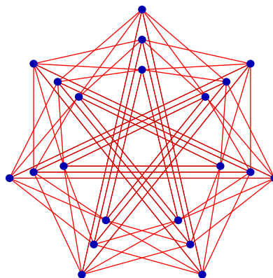
Figure 2: Graph G(3) which arrows \Lambda .
