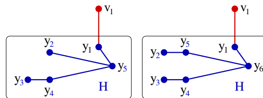
Figure 3: Small graphs, \delta = 1, \Delta = 3 in Lemma 12
