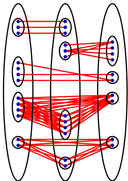
Figure 1: A graph from class \mathcal{P}'_3 .
