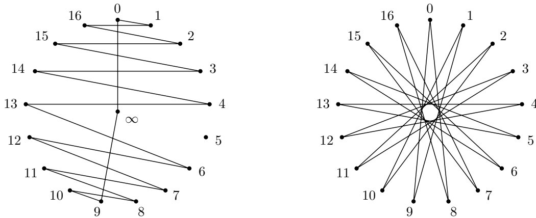
Figure 2: The cycles C and D when k = 17
