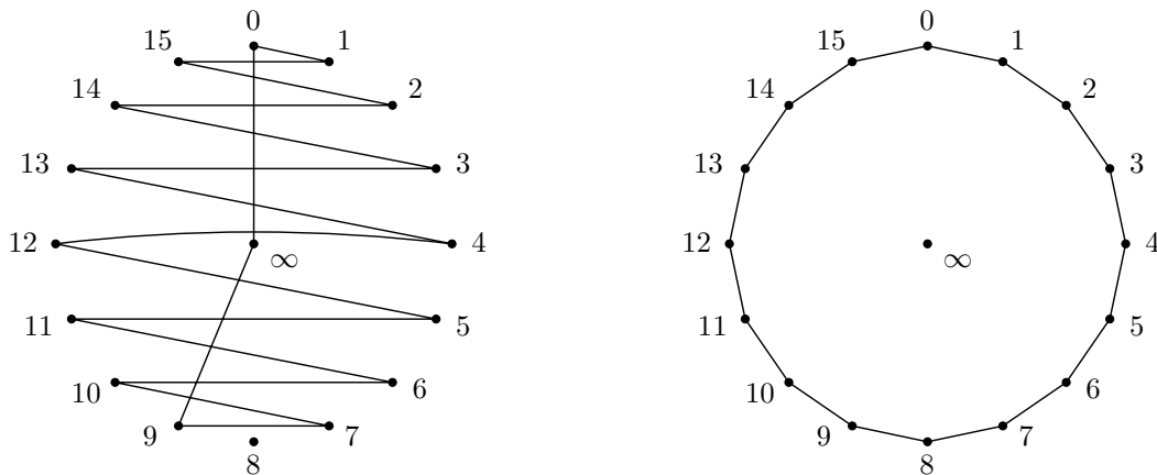
Figure 1: The cycles C and D when k = 16
