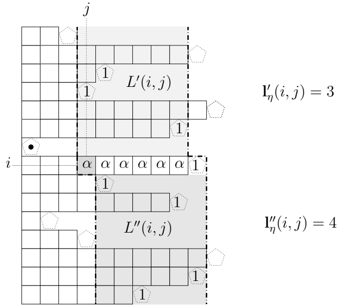
Figure 1: Diagrammatic representation of the \alpha -hooklength of the cell s = (i, j) = (8, 4) . We add a (dotted) pentagonal cell at the end of each row. The three terms 1 + I'_\eta(s) + I''_\eta(s) of the \alpha -hook length count respectively the pentagonal cell of row i , the number of pentagonal cells that belong to the set L'(s) = \{(k, l) \mid k < i \text{ and } j \leq l \leq \eta_i\} and the number of pentagonal cells that belong to L''(s) = \{(k, l) \mid i < k \text{ and } j + 1 \leq l \leq \eta_i + 1\} . The coefficient \mathbf{a}_\eta(s) + 1 of \alpha counts the cells in row i from (i, j) to (i, \eta_i) . In this example we have d_\eta(s) = (1 + 3 + 4) + 6\alpha .
