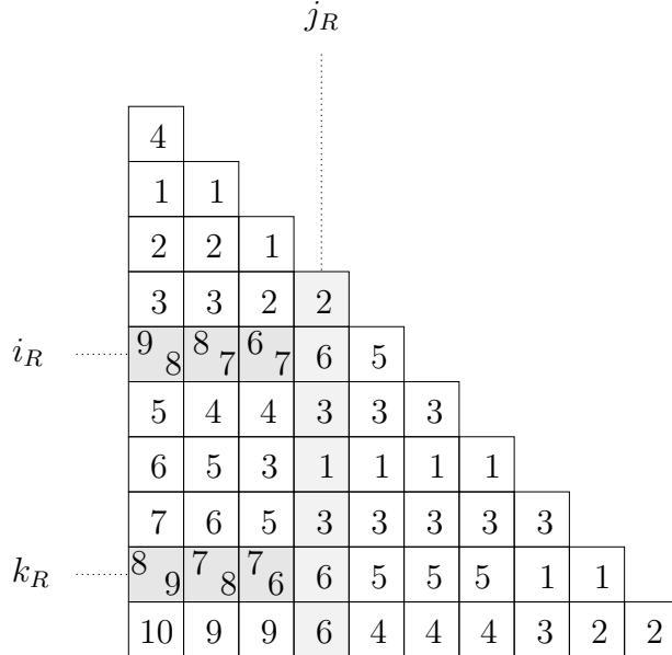
Figure 6: The bijection \Phi illustrated with an example. The triangular tableaux R and T are represented on the same diagram. Labels of R and T , when distinct, are in the upper left corner and lower right corner respectively. For the sake of simplicity we chose \gamma = 0^{m-1} .
