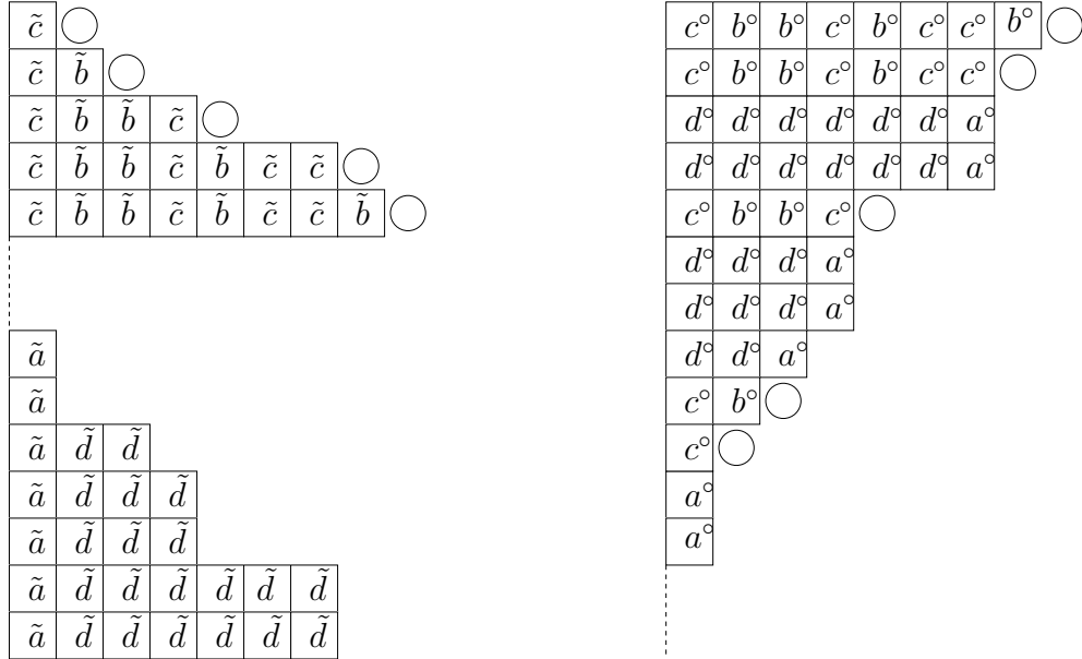
Figure 3: There is a weight preserving bijection between cells of \{\tilde{c}, \tilde{d}\} \subset \tilde{\Lambda} and those of \{c^\circ, d^\circ\} \subset \Lambda^\circ \subset \Lambda^* . Roughly speaking, this bijection corresponds to a sorting of rows according to their length and a cyclic shift of one cell to the left for non-fermionic rows. We denote by W(X) the product of the appropriate weight of the cells in X . The bijection implies then W(\{\tilde{c}, \tilde{d}\}) = W(\{c^\circ, d^\circ\}) , and as a consequence we get \frac{W(\tilde{\Lambda})}{W(\{\tilde{a}\})W(\{\tilde{b}\})} = W(\{\tilde{c}, \tilde{d}\}) = W(\{c^\circ, d^\circ\}) = \frac{W(\Lambda^\circ)}{W(\{a^\circ\})} .
