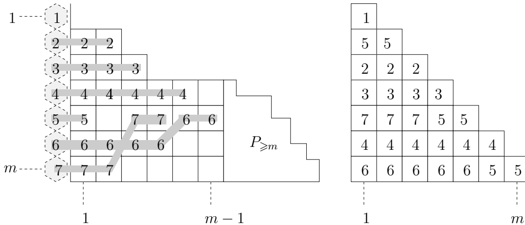
Figure 5: An example of the bijection between \mathcal{G}_{\tilde{\Lambda}} and \mathcal{V}_{\gamma} in the case m = 7 and \gamma = (1, 0, 1, 1, 0, 0) . On the left, we draw the diagrammatic representation of the relevant part of the good- \tilde{\Lambda} configuration P and an additional column 0 of hexagons labeled by the rows' indices. Cells to the right of column m - 1 define a subconfiguration P_{\geq m} whose shape or labels do not contribute to the weight. On the right, we have the element of \mathcal{V}_{\gamma} on which is mapped this configuration. In the configuration, the thick grey line starting from the hexagon labeled by i represents the row \lambda^{(k_i+1)} = (i, i_1, i_2, \dots, i_{k_i}) in the partition.
