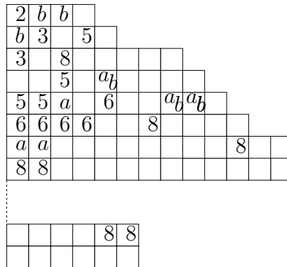
Figure 4: Here are two bad \tilde{\Lambda} -configurations mapped onto each others by the involution. Empty cells implicitly contain a label greater than m (set equal to 8 in the example). In cells with two labels, the labels in the upper left (resp. lower right) corner correspond to the labels of P (resp. P' ). In the example, we have a = 7 , j = 4 , b = 4 . Observe that we can have labels not larger than m in the non-fermionic portion of a \tilde{\Lambda} -configuration. For instance the 8 in column 5 is possible only because there is no 8 in column 4.
