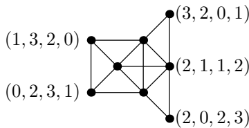
Figure 3: A frame-graph.
