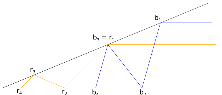
Figure 3: The wedge for j = 1 , the base case for our induction.
