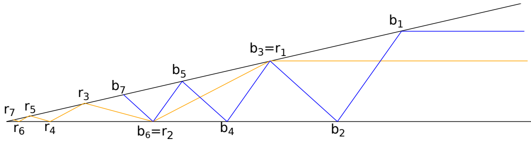
Figure 5: The wedge for j = 2 .
