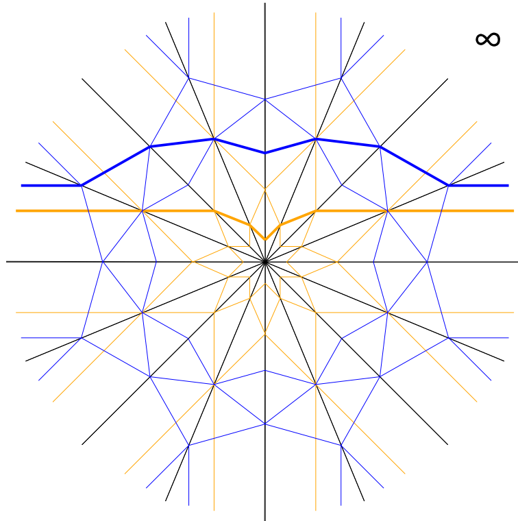
Figure 4: The arrangement for j = 1 , containing 3(6j + 2) + 1 = 25 pseudolines. Each pseudoline is incident to at most 10 vertices.
