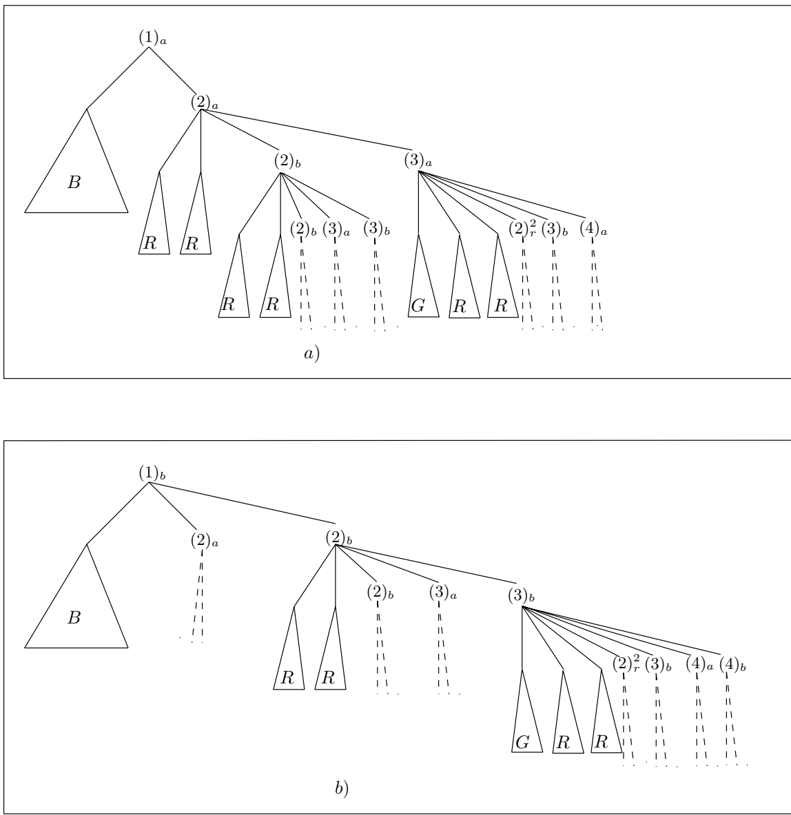
Figure 17: The first levels of the generating trees associated with the rules \Omega(a) , and \Omega''(b) .
