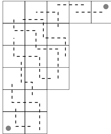
Figure 3: Snakes for the shape 533322
