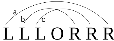
Figure 8: A labelled interval set of the shape 444
