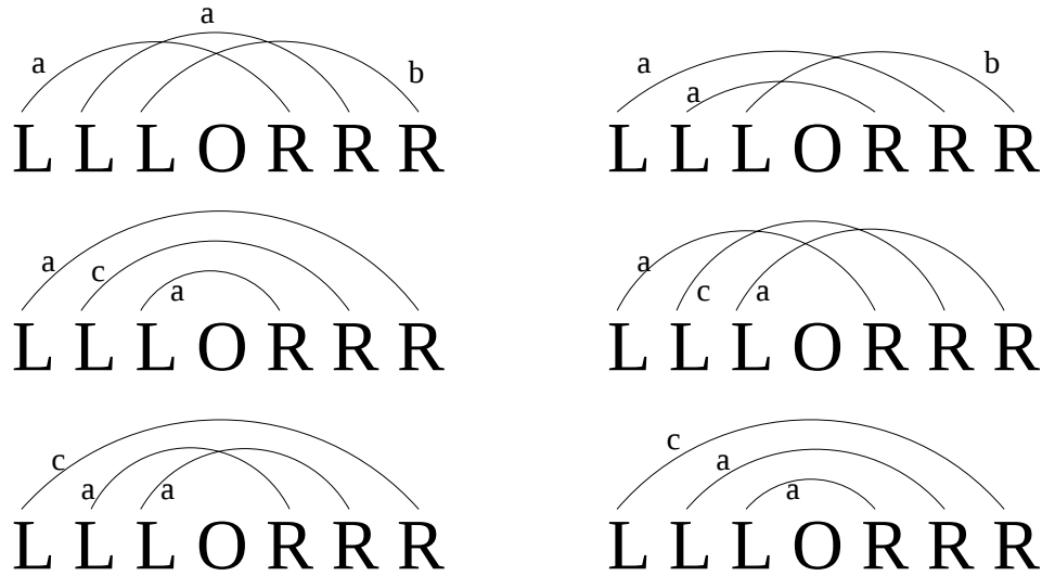
Figure 7: Some labelled interval sets of the shape 444
