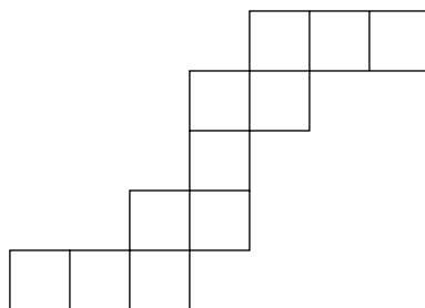
Figure 1: The border strip 75443/4332
