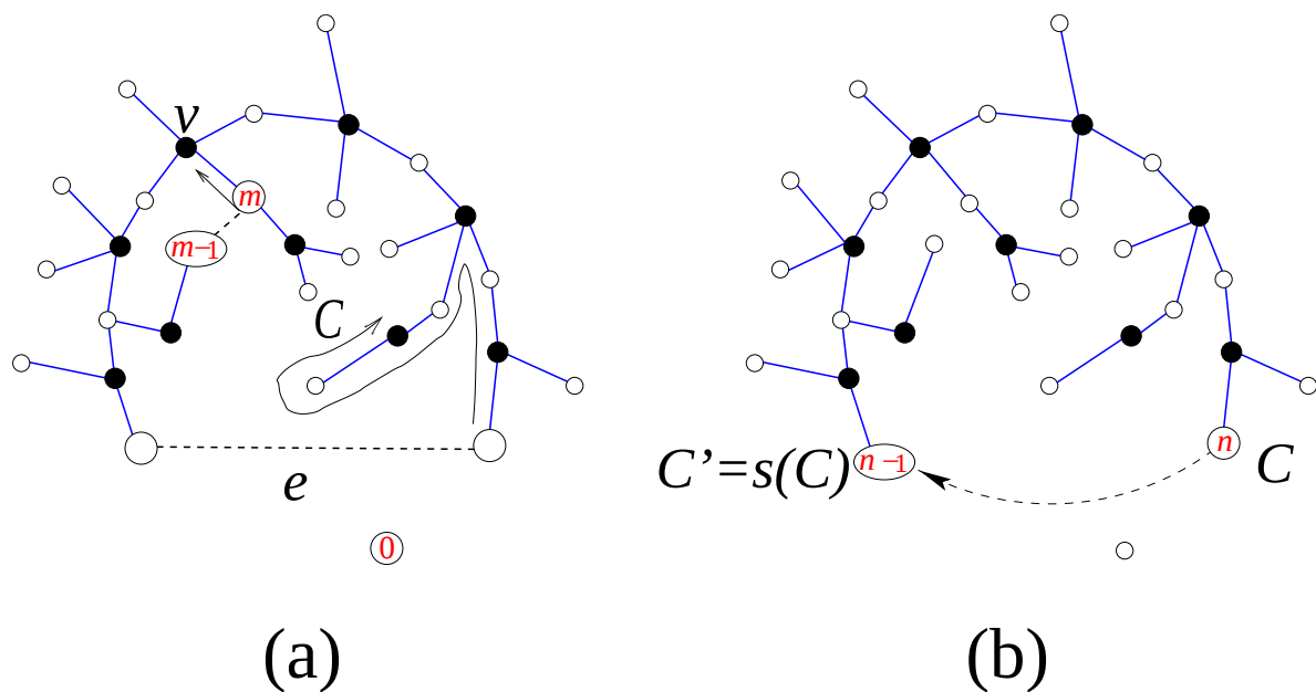
Fig. 5: Proof that any edge e of \mathcal{M} is restored in the construction of section 2.2. Apart from the trivial case where the origin is adjacent to e , the union of e and \mathcal{T} has two faces. We follow (a) counterclockwise the contour path \mathcal{C} bordering the face not containing the origin and pick a corner with smallest label m (represented here with an outgoing arrow). If this corner were not the last one on \mathcal{C} (adjacent to e ), it would be followed by an unlabeled vertex v and by the selection rules of figure 1 around v , we would deduce the existence of another corner with label m - 1 inside the face. As the face does not contain the origin, the corner m - 1 is different from the origin hence it lies on the contour \mathcal{C} , a contradiction. This implies (b) that the end corner of \mathcal{C} is the successor of its starting corner, hence that e is restored.
