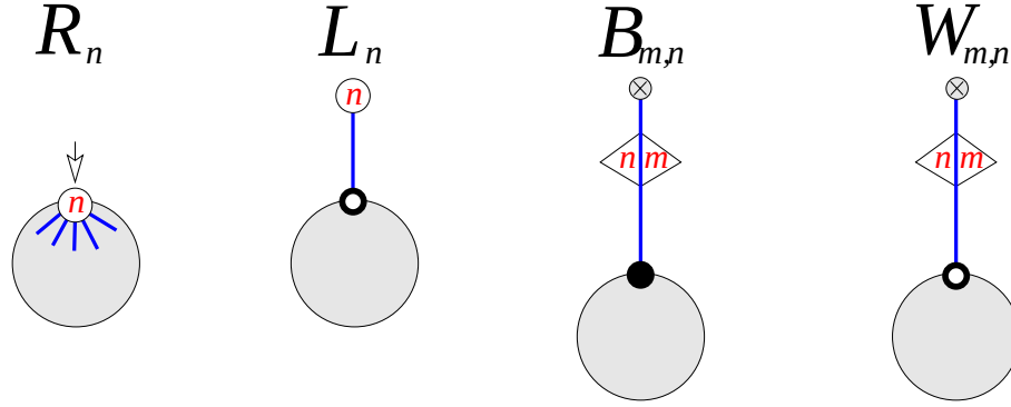
Fig. 14: The generating functions R_n, L_n, B_{m,n}, W_{m,n} for respectively rooted mobiles with root corner labeled n , rooted mobiles with univalent root vertex labeled n , and half-mobiles with unlabeled univalent root vertex attached to a flagged edge with labels n, m incident to a black, white vertex.
