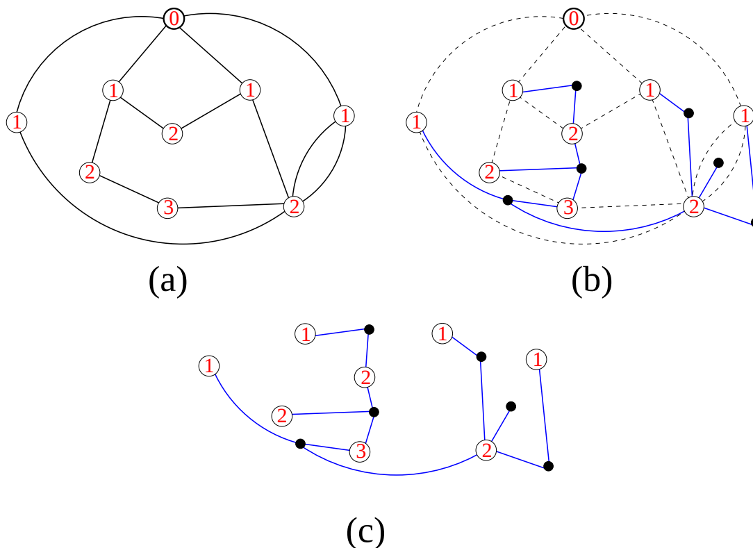
Fig. 3: A typical example of a planar map \mathcal{M} (a) with one 2-valent, three 4-valent and two 6-valent faces. Having selected an origin (labeled 0), all the vertices are naturally labeled by their geodesic distance to that origin. We perform (b) the construction of figure 1 in each face of \mathcal{M} (with, as usual, the opposite conventions for the external face due to the representation in the plane). Erasing the original edges of \mathcal{M} as well as its origin, we are left (c) with a tree \mathcal{T} .
