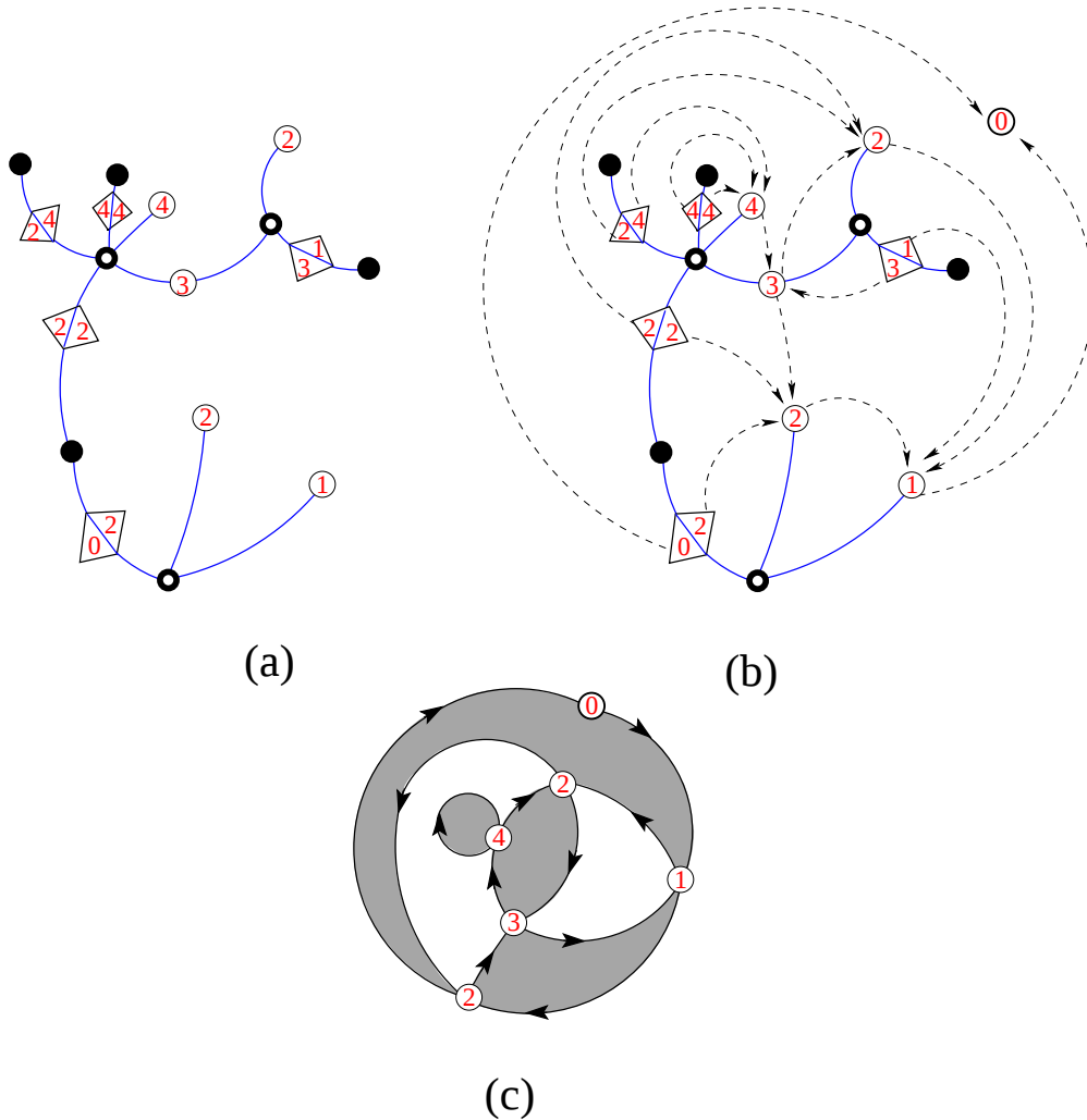
Fig. 13: The construction of an Eulerian map \mathcal{M} with an origin out of a sample well-labeled generalized mobile \mathcal{T} . Starting from the mobile (a) we connect each labeled corner and flag to its successor via an oriented edge (dashed arrow). This includes adding a vertex labeled 0, successor of all corners labeled 1 and flags labeled 0. Erasing all unlabeled vertices and all edges of the mobile produces an Eulerian planar map with an origin (c). Its vertex labels moreover encode their geodesic distance from the origin.
