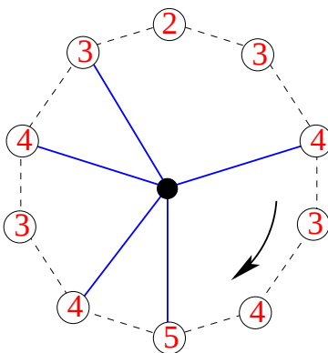
Fig. 1: A typical configuration of labels around a face of \mathcal{M} (delimited by dashed edges), here of valence 2k = 10 . Adjacent labels differ by \pm 1 . We add a black unlabeled vertex at the center of the face and connect it (via solid edges) to the k = 5 labeled vertices immediately followed clockwise by a smaller label.
