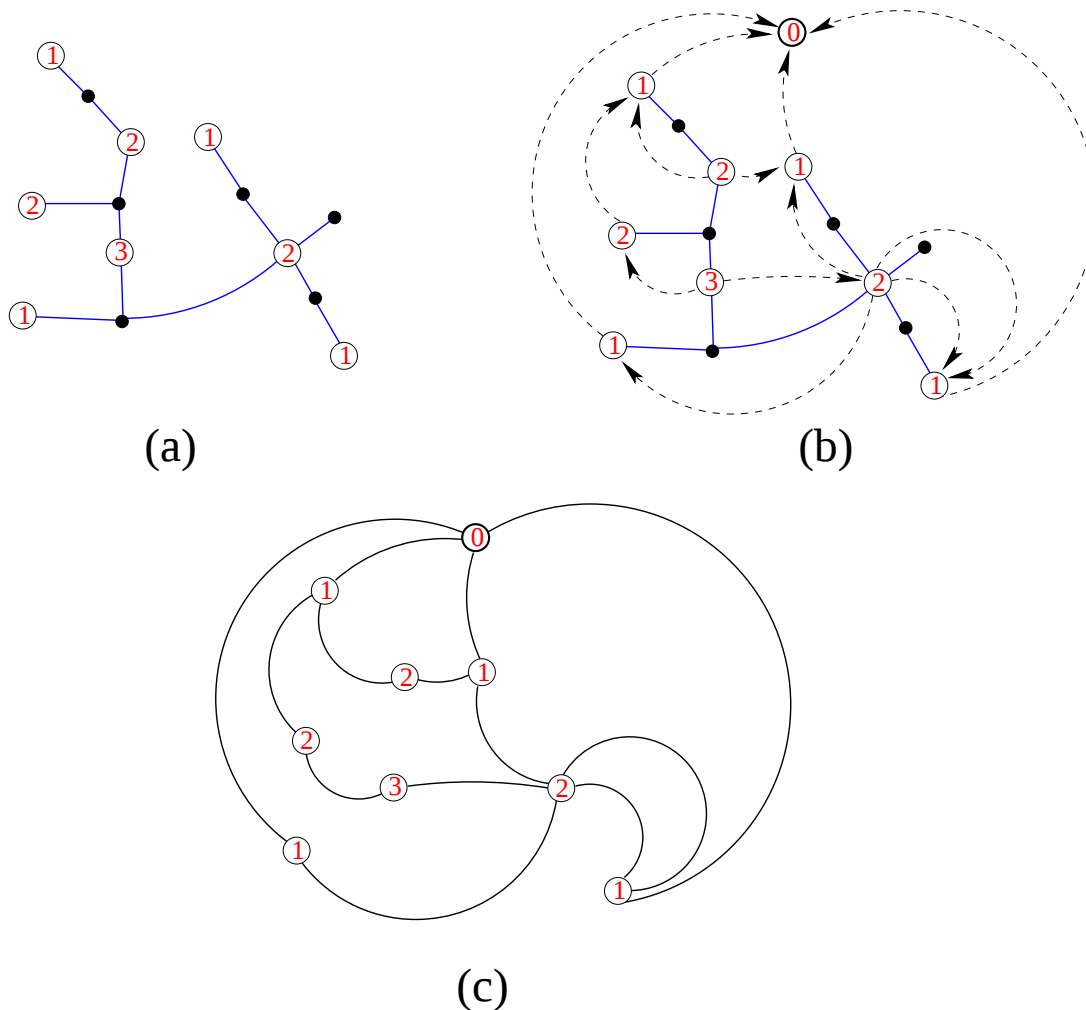
Fig. 4: A typical example of a well-labeled mobile \mathcal{T} (a). For each unlabeled vertex of \mathcal{T} , the successive labels of its adjacent labeled vertices cannot decrease by more than 1 clockwise. We add an extra origin vertex labeled 0 and connect (b) each labeled corner to its successor (dashed arrows). Erasing all unlabeled vertices of \mathcal{T} and their adjacent edges, we are left (c) with a bipartite planar map \mathcal{M} . Moreover, the labels simply encode the geodesic distance from the origin to the vertices.
