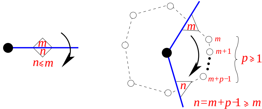
Fig. 10: Constraints P_{\bullet} on labels around a black unlabeled vertex. Clockwise around the vertex two successive (flag) labels m and n must either satisfy n \leq m if the flags share the same edge, or n \geq m otherwise. In the latter case, p = n - m + 1 may be interpreted as the number of labeled vertices incident in \mathcal{M} to the corresponding black face, and in between the two flags.
