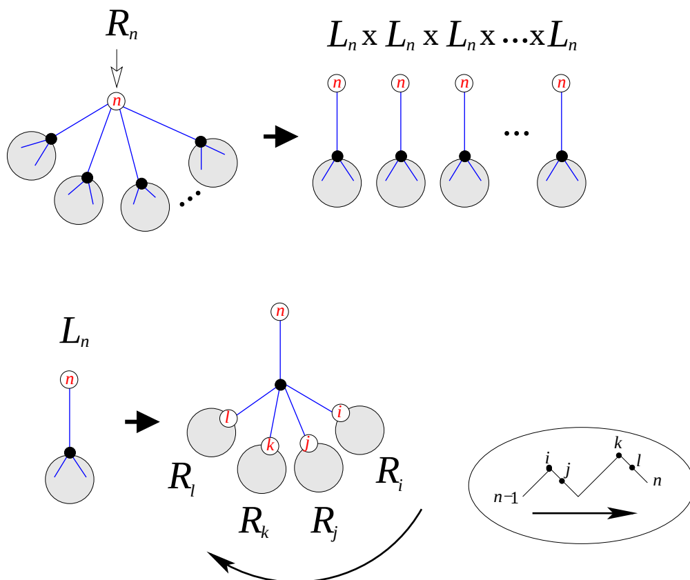
Fig. 7: Top: the decomposition of a rooted mobile with root label n (generating function R_n ) into a number of mobiles with univalent root vertex with the same label (generating function L_n ) leads to eq. (2.1). Bottom: A mobile with univalent root vertex with label n is in turn decomposed according to the clockwise neighborhood of the adjacent unlabeled vertex, in correspondence with walks (see oval). Each descending step i \rightarrow i - 1 on the walk gives rise to a factor R_i for the associated rooted sub-mobile, leading to eq. (2.2).
