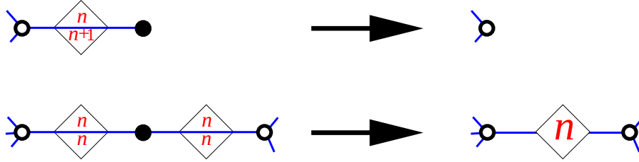
Fig. 16: The two possible situations around an unlabeled black vertex associated with a two-valent black face in an Eulerian map. The arrows indicate simplification rules for the mobiles associated to planar maps with arbitrary valences.
