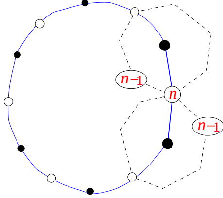
Fig. 2: Proof by contradiction that \mathcal{T} has no cycle. Assuming the existence of such a cycle, we pick a labeled vertex with minimal label n on the cycle. The neighborhoods of its two adjacent unlabeled vertices on the cycle show the existence of a vertex labeled n - 1 on each side of the cycle. A path on \mathcal{M} from the origin to one of these vertices must cross the cycle at a labeled vertex with label at most n - 1 , a contradiction.
