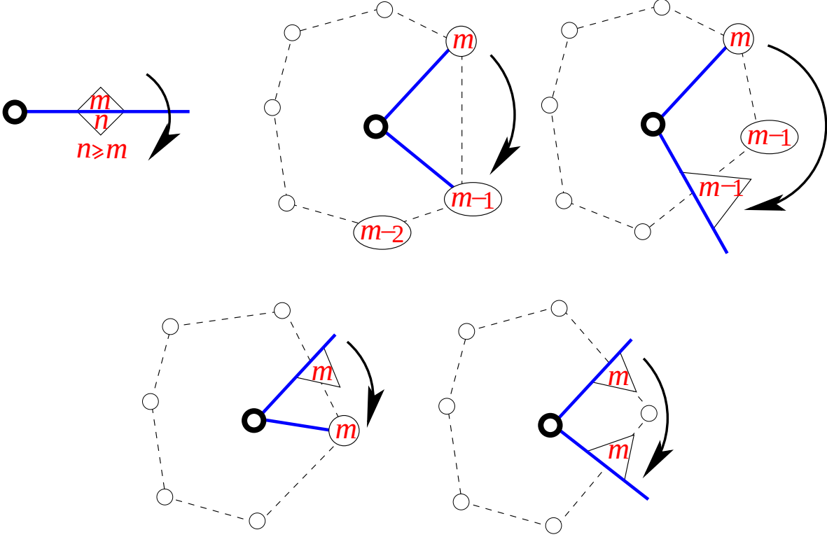
Fig. 11: Constraints P_0 on labels around a white unlabeled vertex read clockwise. Two successive flag labels m and n sharing the same edge must satisfy n \geq m . For consecutive edges, a vertex labeled m is followed by a label m - 1 (either on a vertex or a flag), while a flag labeled m is followed by a label m (either on a vertex or a flag).
