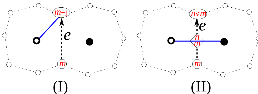
Fig. 8: Rules to construct a tree \mathcal{T} out of an Eulerian map \mathcal{M} . We first add an unlabeled vertex at the center of each face of the map, with the same color (white or black), represented by thick (empty or filled) circles. Each oriented edge e of \mathcal{M} must connect vertices with labels of the form (I) m \rightarrow m + 1 or (II) m \rightarrow n , with n \leq m . Accordingly, we draw an edge of \mathcal{T} respectively connecting (I) the white unlabeled vertex on the left of e to the vertex labeled m + 1 and (II) the white and black unlabeled vertices on both sides of e . In the latter case we decorate the edge with labeled flags carrying the labels of the closest vertices.
