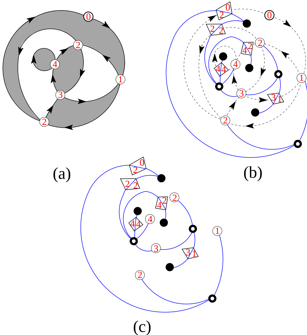
Fig. 9: The construction of a tree \mathcal{T} out of a sample Eulerian map \mathcal{M} with an origin. (a) Each vertex of \mathcal{M} is labeled by its oriented geodesic distance from the origin 0. (b) We perform the construction of figure 8 (I)-(II) for each oriented edge of the map. (c) Erasing the origin and the original edges of \mathcal{M} produces a tree \mathcal{T} carrying labels on some vertices and edges.
