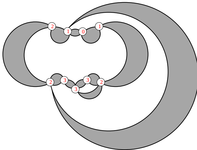
Fig. 15: A sample planar map with arbitrary valences and an origin. The edges are inflated into two-valent black faces producing an Eulerian planar map with only two-valent black faces. As usual, vertices are labeled by their geodesic distance from the origin. The orientation of the edges becomes irrelevant.
