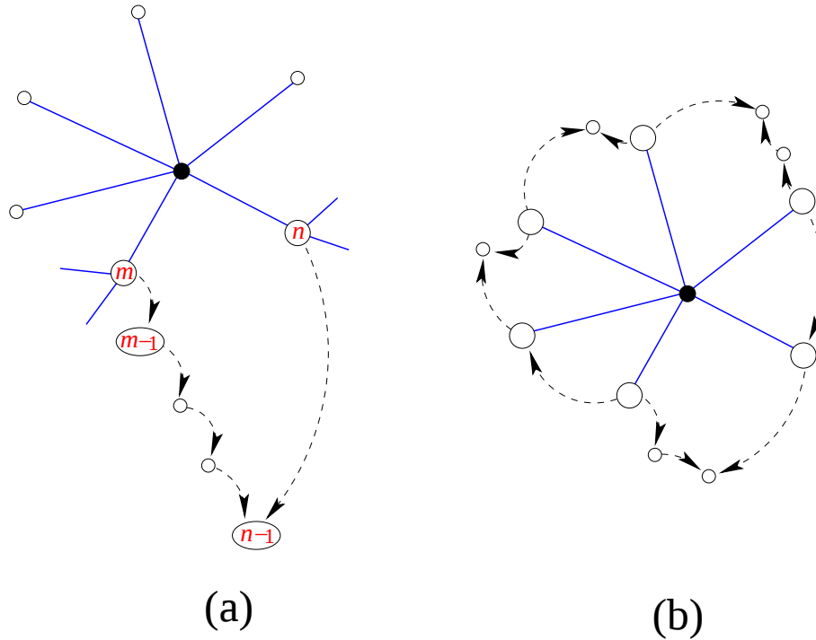
Fig. 6: The generic configuration (a) of successors of two consecutive vertices adjacent to a given unlabeled vertex of \mathcal{T} . Each face of \mathcal{M} is obtained (b) as the union around an unlabeled vertex of all such configurations. As the labels decrease by one along the arrows, we immediately see that the labels of \mathcal{T} are re-selected by the construction of section 2.1 acting on \mathcal{M} .
