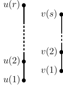
Figure 1: P_{u,v}
