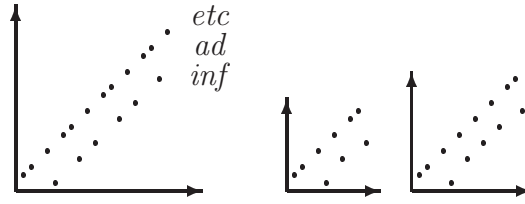
Figure 4: On the left, an infinitely based periodic natural class. On the right, two basis elements.
