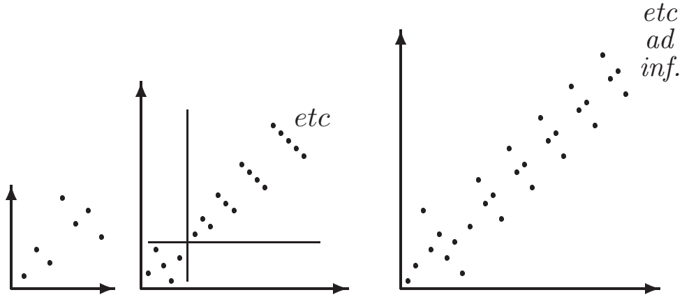
Figure 1: The sum of 132 and 4231 is 1327564, as plotted on the left. Every finitely based natural class is defined by a finite permutation summed with a sum-complete class (centre), or is eventually periodic (right).
