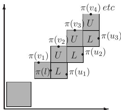
Figure 3: \pi mapped out by u_i and v_i . None of the boxes marked L or U contains a monotonic increasing or decreasing subsequence of length b . Thus the sizes of these boxes is bounded.
