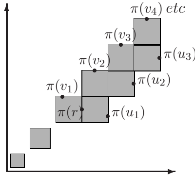
Figure 2: The terms of \pi as mapped out by \pi(u_i) and \pi(v_i) . All terms lie in the shaded boxes.
