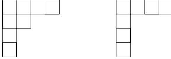
Figure 2: Reinforced hooks such as (4,2,1,1) are not rank-maximal, but ordinary hooks such as (4,1,1,1) are.
