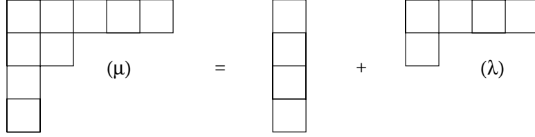
Figure 1: \mu extends \lambda , where \mu = (5, 2, 1, 1) , \lambda = (4, 1) , and \mu - \lambda = (1, 1, 1, 1) .
