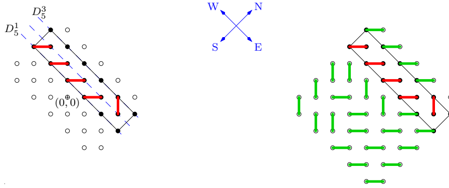
Figure 11: Left: the W-E Aztec tube of size 5 with b = 1 and t = 3 , and a quasi-matching. Right: extension of this quasi-matching to a matching of an Aztec diamond of size 5.
