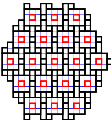
Figure 18: Extending the embedding of the 4-6-12 (semi-)regular tessellation in order to make it gapless.
