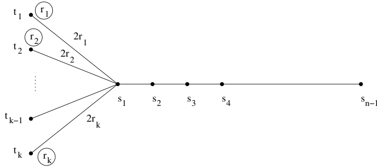
Figure 1: The “Dynkin diagram” of G_{r_1, \dots, r_k; n}
