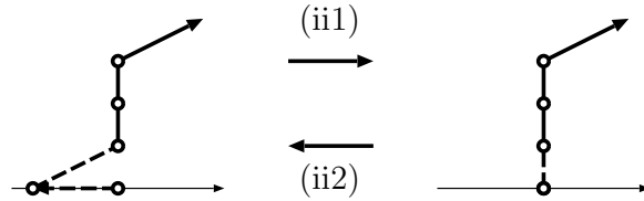
Figure 7: Transformations by T_{1,4}^{S \times F} , Case (ii).
