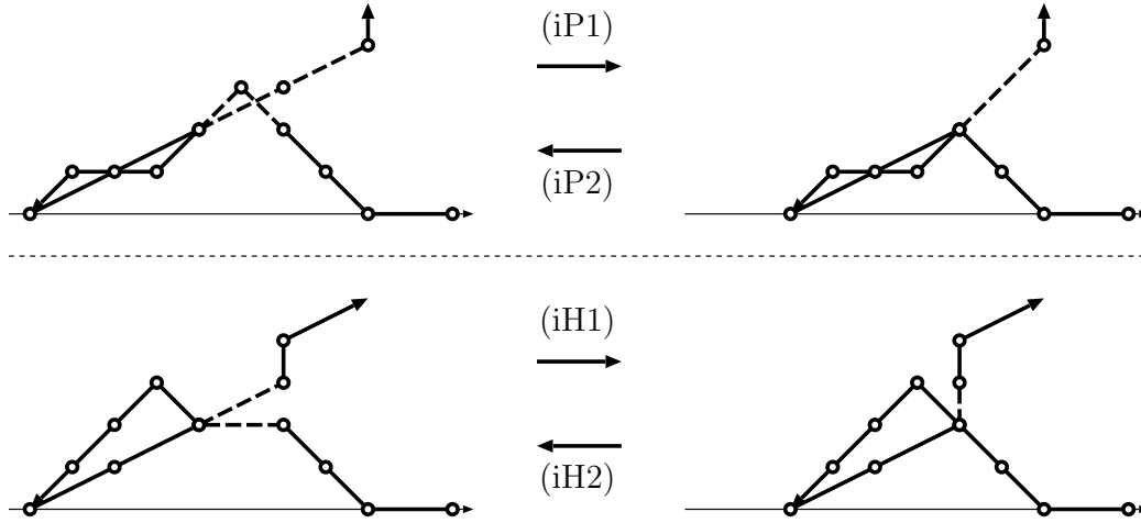
Figure 6: Transformations by T_{-1,5}^{S \times F} , Case (i).
