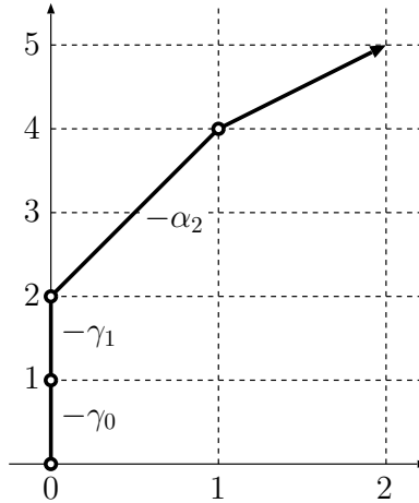
Figure 2: A Favard-LBP path \eta = c_0^F c_1^F a_2^F b_4^F of height 5 and width 2, \text{wgt}(v; \eta) = -\alpha_2 \gamma_0 \gamma_1 .
