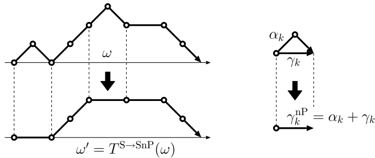
Figure 9: A transformation by T^{\text{S} \rightarrow \text{SnP}} .
