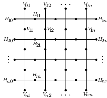
Figure 1: Assignment of edge matrix entries to lattice edges.
