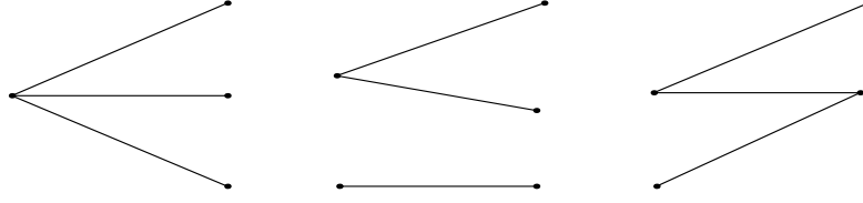
Figure 3: The 3 edge subgraphs
