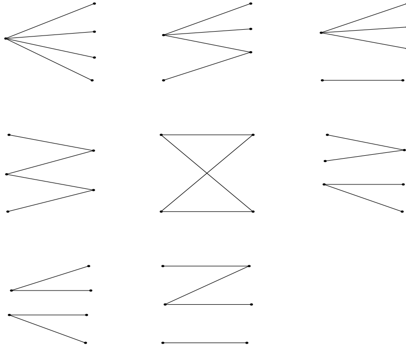
Figure 4: The 4 edge subgraphs
