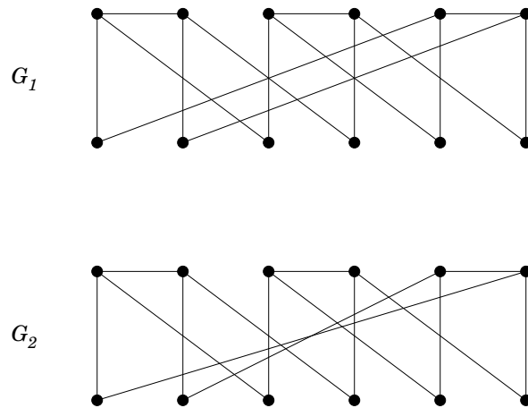
Figure 39: graphs arising from H = K_2 \cup K_2 \cup K_2 in Proposition 3.15
