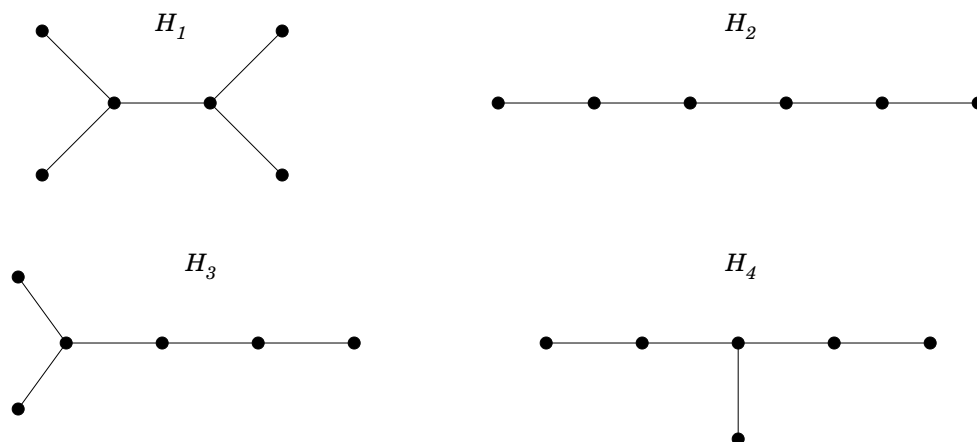
Figure 30: choices for H when n = 10, a = 4 in Proposition 3.15
