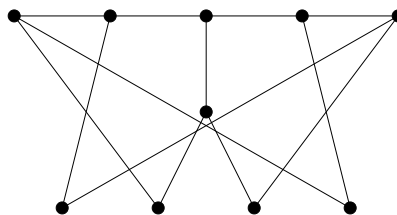
Figure 34: graph arising from H_4 in Proposition 3.15
