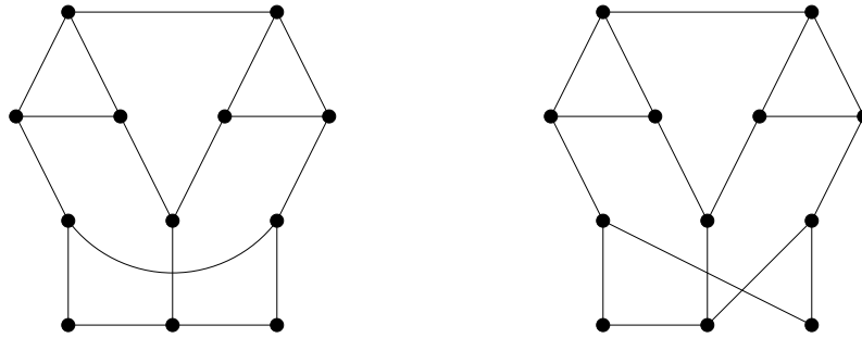
Figure 58: graphs arising from G_2 in Proposition 3.17 when n = 12
