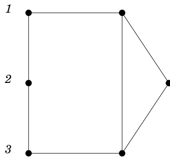
Figure 10: graph on 6 vertices from Lemma 3.5
