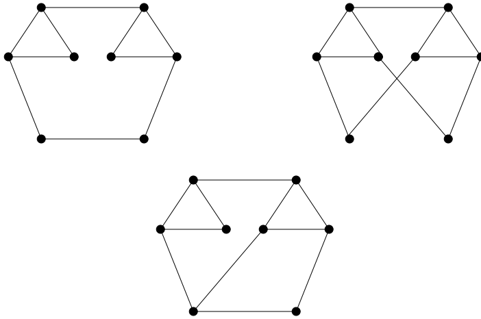
Figure 26: graphs in Remark 3.11
