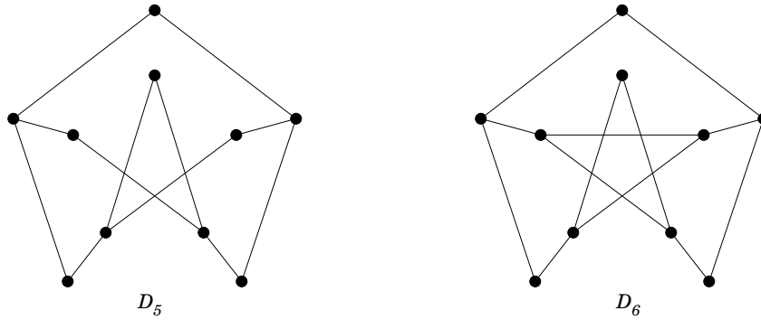
Figure 60: alternative drawings of D_5 and D_6
