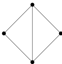
Figure 13: the induced subgraph in Lemma 3.6
