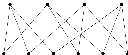
Figure 29: Laplacian integral graph of Proposition 3.15 with n = 10, a = 6
