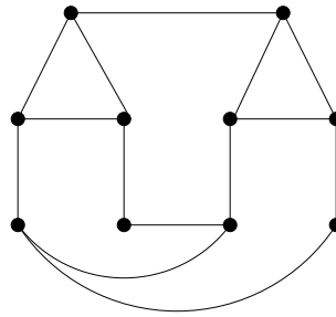
Figure 56: graph arising from G_1 in Proposition 3.17 when n = 10
