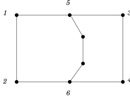
Figure 9: graph on 8 vertices from Lemma 3.4
