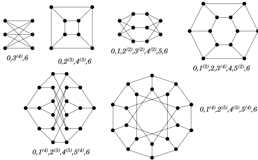
Figure 1: 3-regular, bipartite, Laplacian integral graphs
