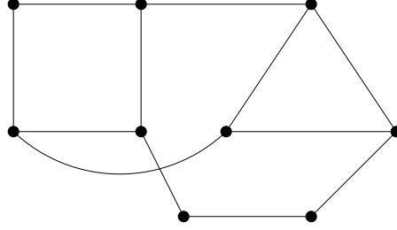
Figure 49: subgraph giving rise to a cutpoint in Proposition 3.16
