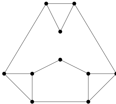
Figure 21: graph with n = 10 in Lemma 3.9
