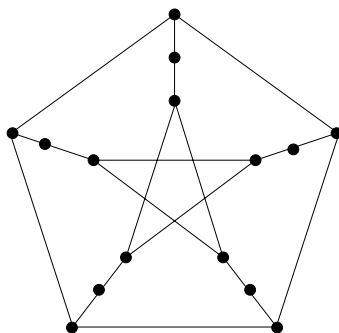
Figure 28: Laplacian integral graph of Proposition 3.15 with n = 15, a = 5
