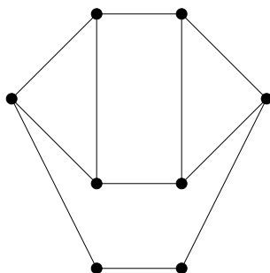
Figure 18: graph with n = 8 in Lemma 3.8
