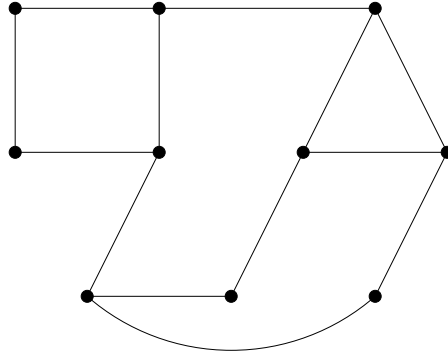
Figure 50: graph for n = 10 with adjacent vertices of degree 2 on the 4-cycle
