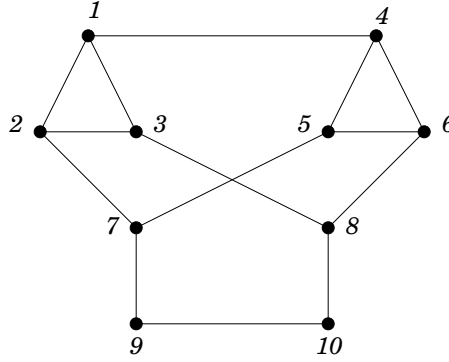
Figure 55: graph arising if G_3 is a subgraph in Proposition 3.17
