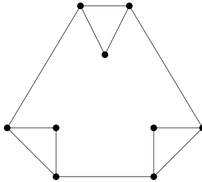
Figure 20: induced subgraph in Lemma 3.9
