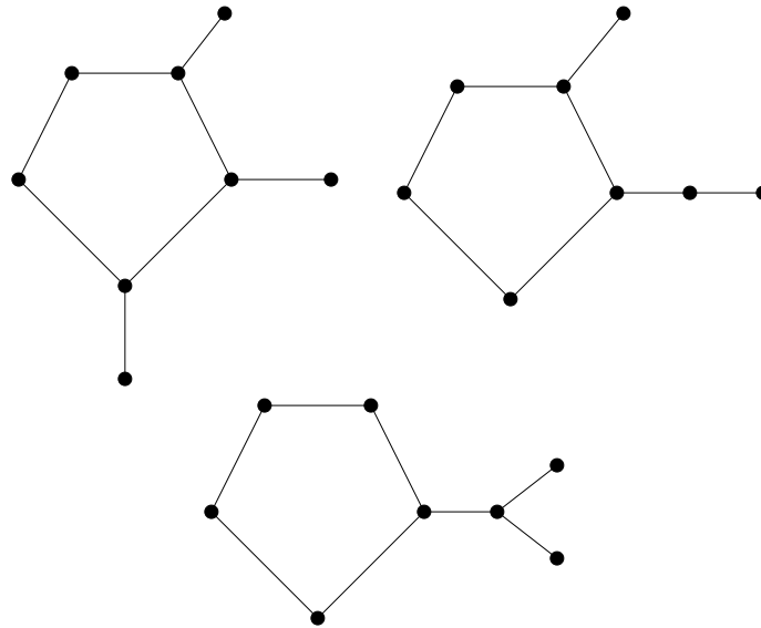
Figure 42: graphs in Proposition 3.15 with \lambda_{min} < -2
