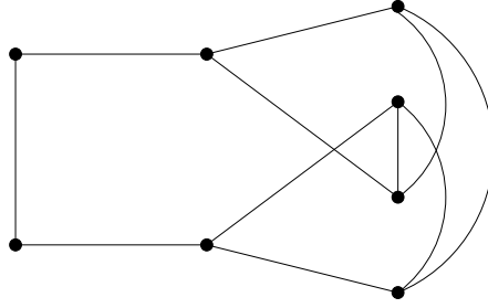
Figure 7: illustration of conclusion b) in Lemma 3.1
