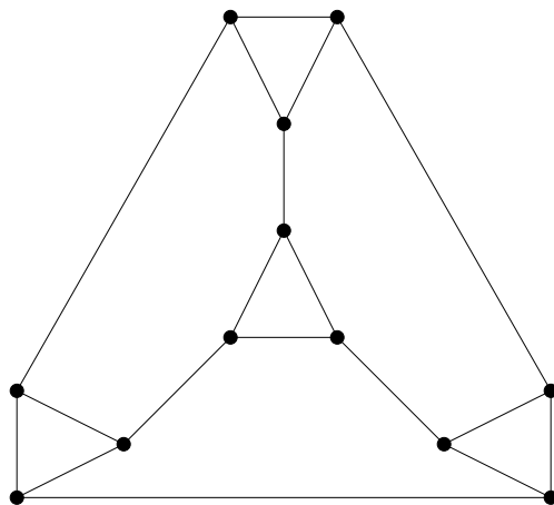
Figure 19: cubic graph in Lemma 3.9
