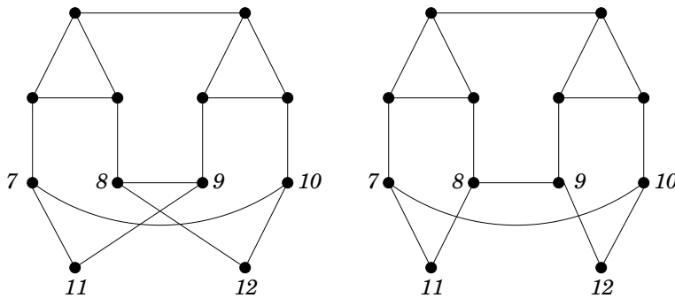
Figure 59: graphs arising from G_1 in Proposition 3.17 when n = 12
