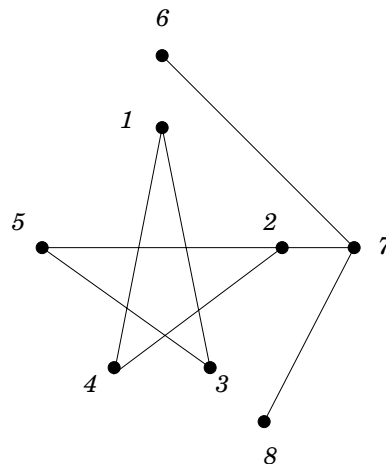
Figure 35: subgraph of H when n = 10, a = 2 in Proposition 3.15
