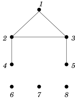
Figure 24: subgraph in Lemma 3.10
