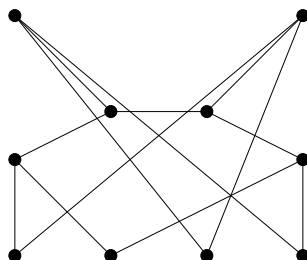
Figure 31: Laplacian integral graph for n = 10, a = 4 in Proposition 3.15
