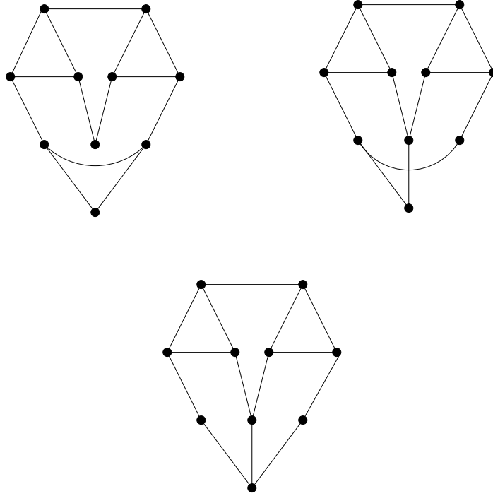
Figure 57: graphs arising from G_2 in Proposition 3.17 when n = 10
