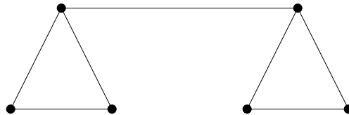
Figure 53: subgraph in Proposition 3.17
