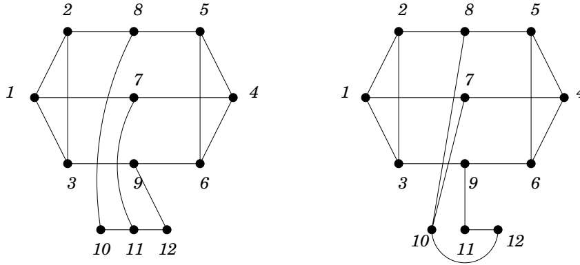
Figure 16: graphs with n = 12 from Lemma 3.7
