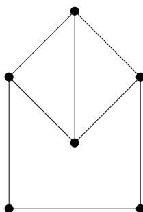
Figure 14: the graph for case that n = 6 in Lemma 3.6
