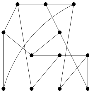
Figure 45: graph arising from H_6 in Proposition 3.15
