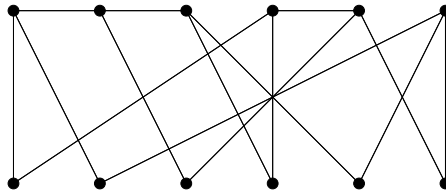
Figure 38: graph in Proposition 3.15 arising from H = P_3 \cup K_2 \cup K_1
