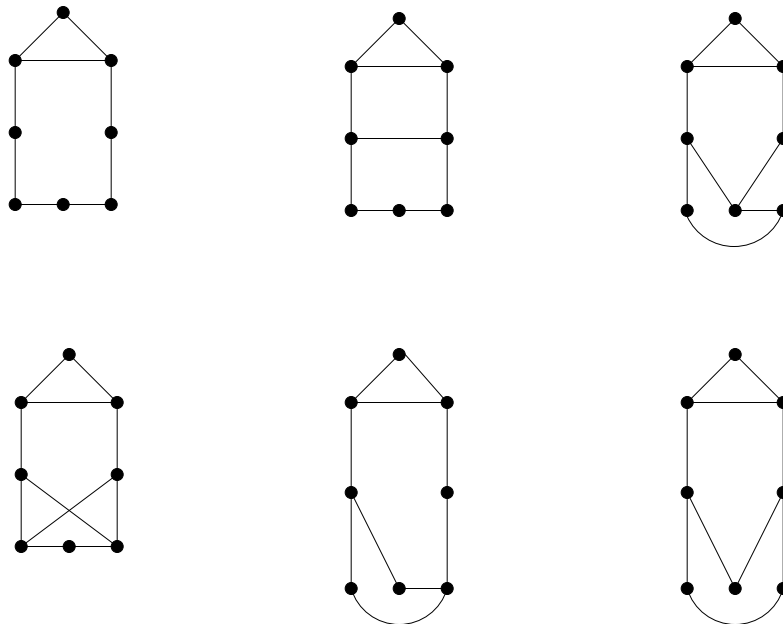
Figure 25: graphs with n = 8 in Lemma 3.10
