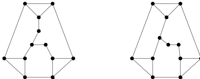
Figure 22: graphs with n = 12 in Lemma 3.9
