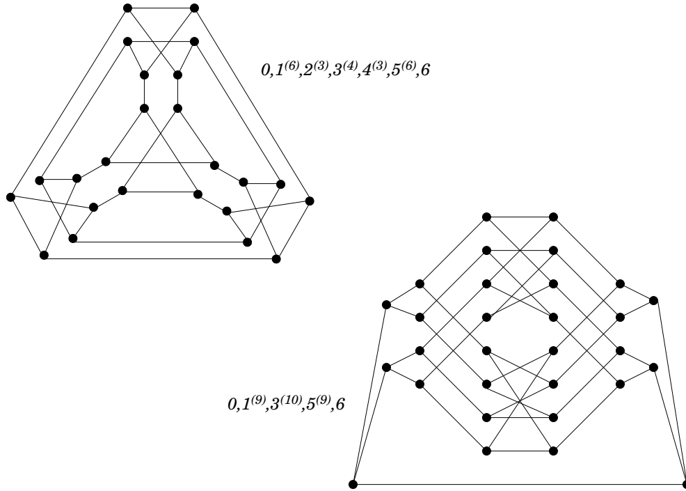
Figure 2: 3-regular, bipartite, Laplacian integral graphs
