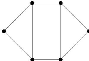
Figure 17: Laplacian integral graph from Lemma 3.8
