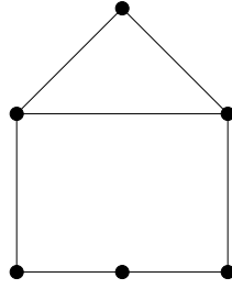
Figure 23: graph with n = 6 in Lemma 3.10
