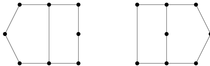
Figure 11: graphs from Lemma 3.5 with six vertices of degree 2
