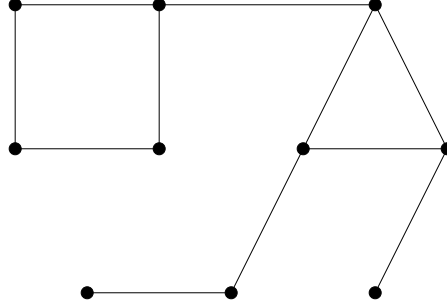
Figure 51: subgraph when there are no adjacent vertices of degree 2 on the 4-cycle
