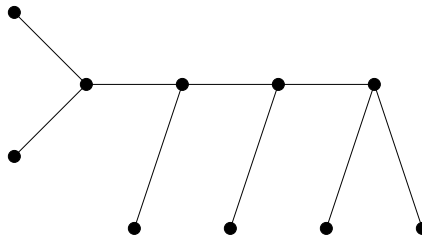
Figure 33: subgraph arising from H_3 in Proposition 3.15
