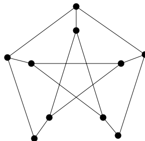
Figure 36: Laplacian integral graph for n = 10, a = 2
