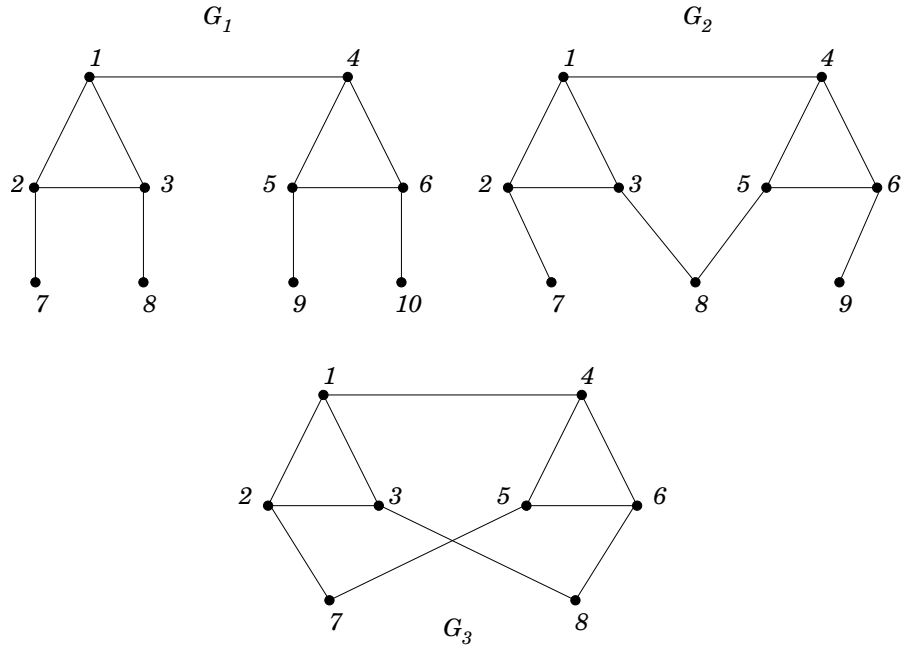
Figure 54: the subgraphs G_1, G_2, G_3 in Proposition 3.17
