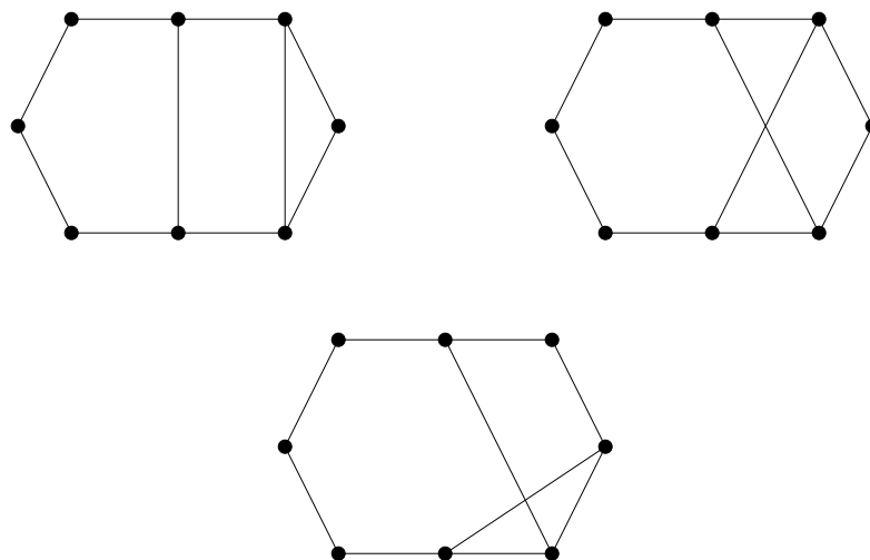
Figure 12: graphs from Lemma 3.5 with four vertices of degree 2
