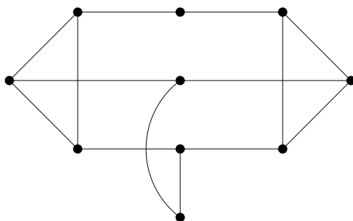
Figure 15: Laplacian integral graph from Lemma 3.7
