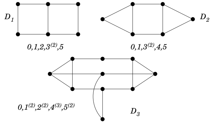
Figure 4: connected, non-regular, Laplacian integral graphs with maximum degree 3
