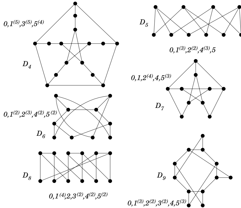
Figure 5: connected, non-regular, Laplacian integral graphs with maximum degree 3
