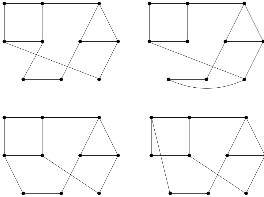
Figure 52: choices for G in Proposition 3.16
