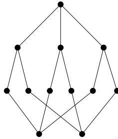
Figure 37: graph arising when H = K_{1,3} \cup \overline{K_2}
