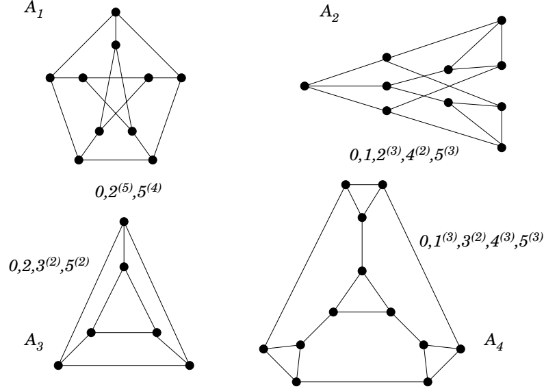
Figure 3: 3-regular, non-bipartite, Laplacian integral graphs
