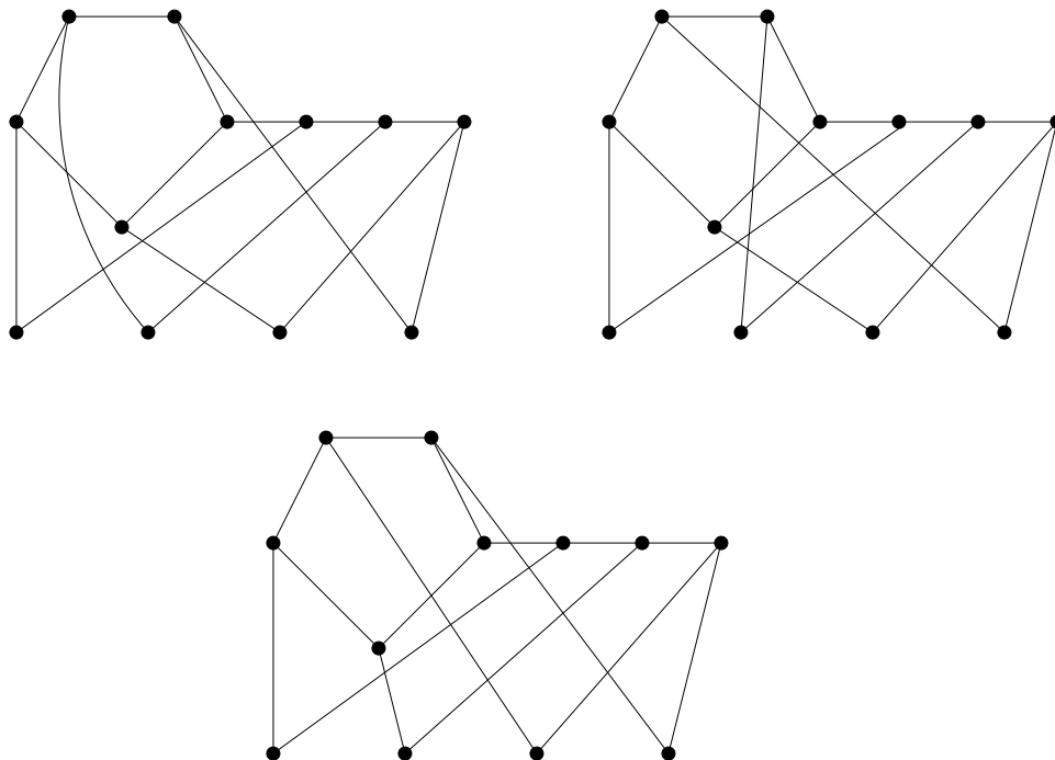
Figure 46: graphs arising from H_7 in Proposition 3.15
