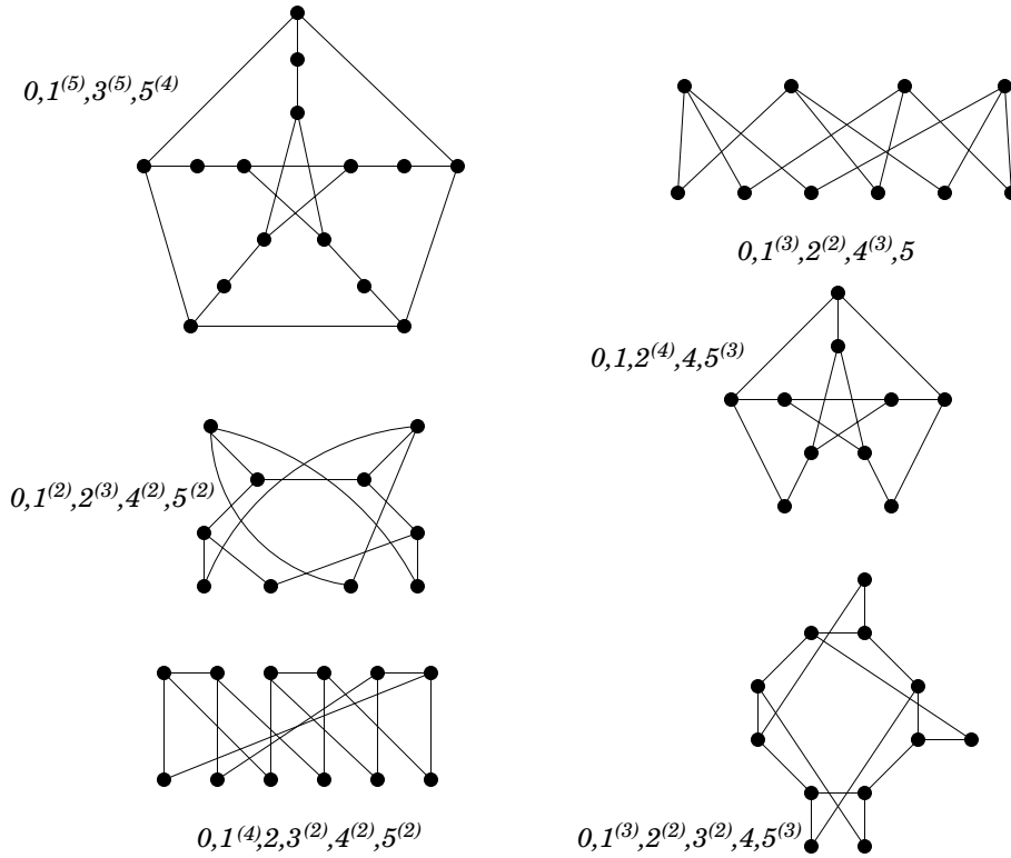
Figure 27: Laplacian integral graphs for Proposition 3.15
