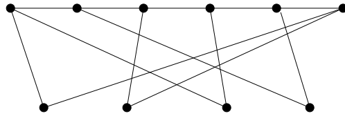
Figure 32: graphs arising from H_2 in Proposition 3.15
