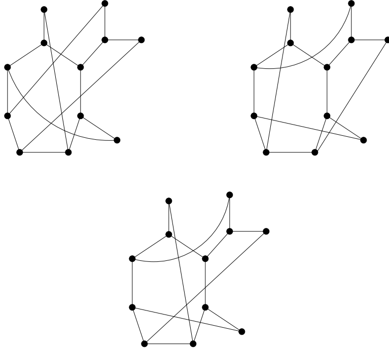
Figure 41: graphs arising if H contains a C_7 in Proposition 3.15
