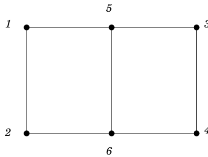
Figure 8: graph on 6 vertices from Lemma 3.4
