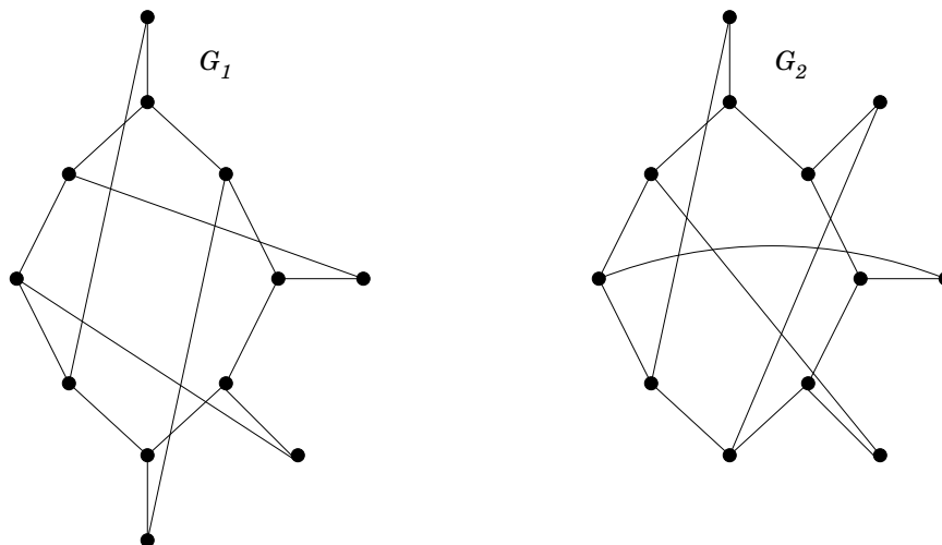
Figure 40: graphs arising from H = C_8 in Proposition 3.15
