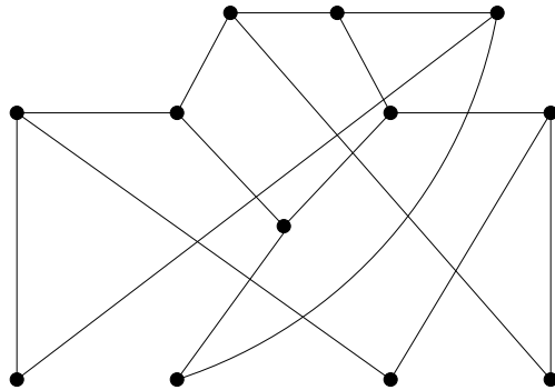
Figure 44: graph arising from H_5 in Proposition 3.15
