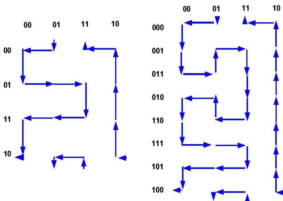
Figure 2: Balanced cyclic 4- and 5-digit binary Gray codes.
