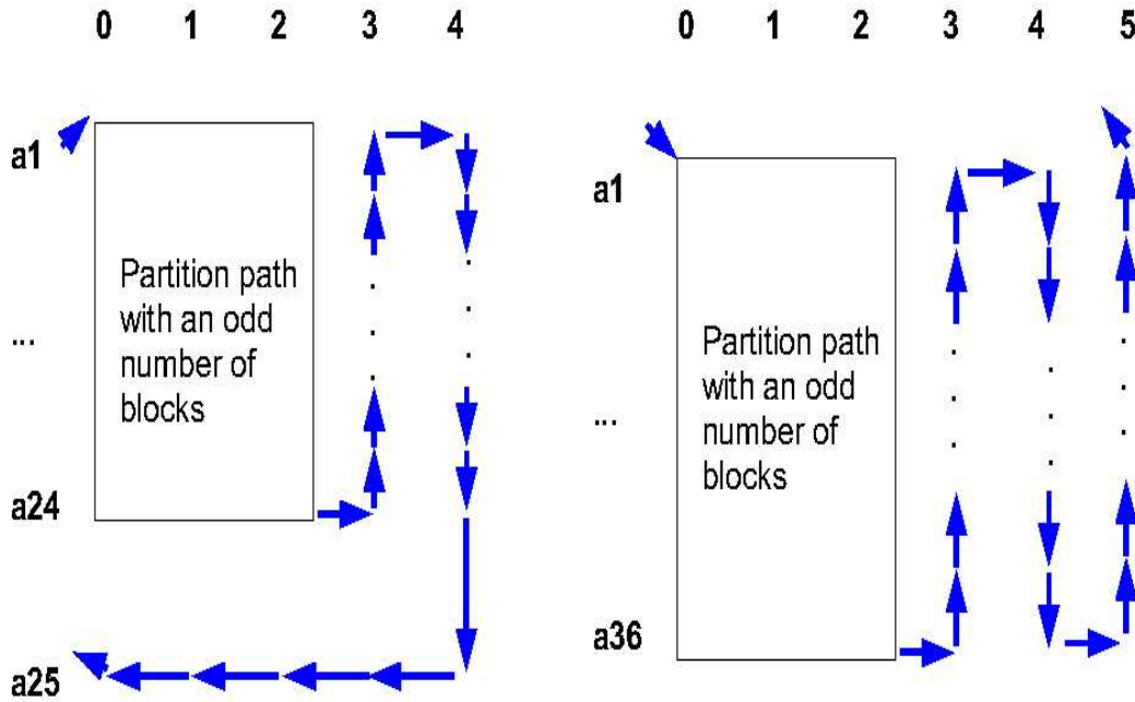
Figure 3: The structure of 3-digit codes for R = 3 \cdot 1 + 2 and R = 3 \cdot 1 + 3 .
