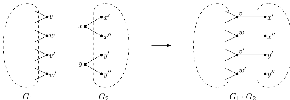
Figure 1: The dot product construction
