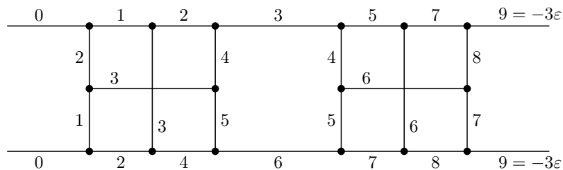
Figure 4: The colouring of two consecutive B -blocks of B_n^2 used in the proof of Lemma 3. All colours are negated for better readability.
