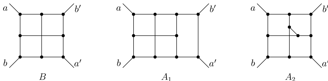
Figure 2: The Blanuša blocks
