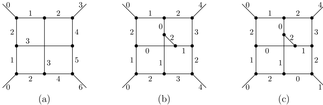
Figure 3: Consecutive colourings of Blanuša blocks used in Lemma 3.
