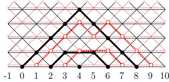
Figure 5: A configuration of Schröder paths with sources \{(2j, 0); j = 0, 1, 2, 3, 4\} and sinks \{(2j, 0); j = 0, 1, 2, 4, 5\} .
