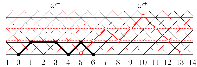
Figure 1: Schröder paths \omega^- (the left one on G^- ) and \omega^+ (the right one on G^+ ) on G .
