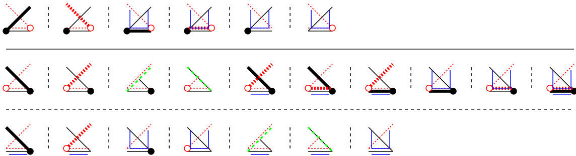
Figure 9: Possible pieces (before gluing).
