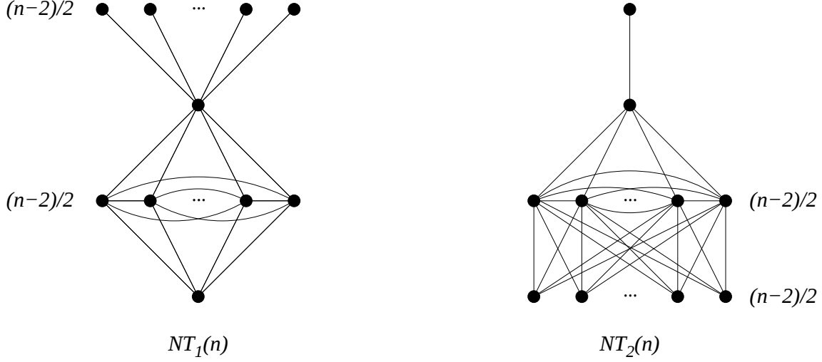
Figure 3: Two NT graphs
