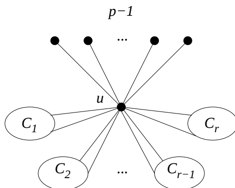
Figure 1: Connected components at u
