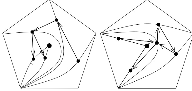
Figure 4: Some examples of triangulations and corresponding quiver.
