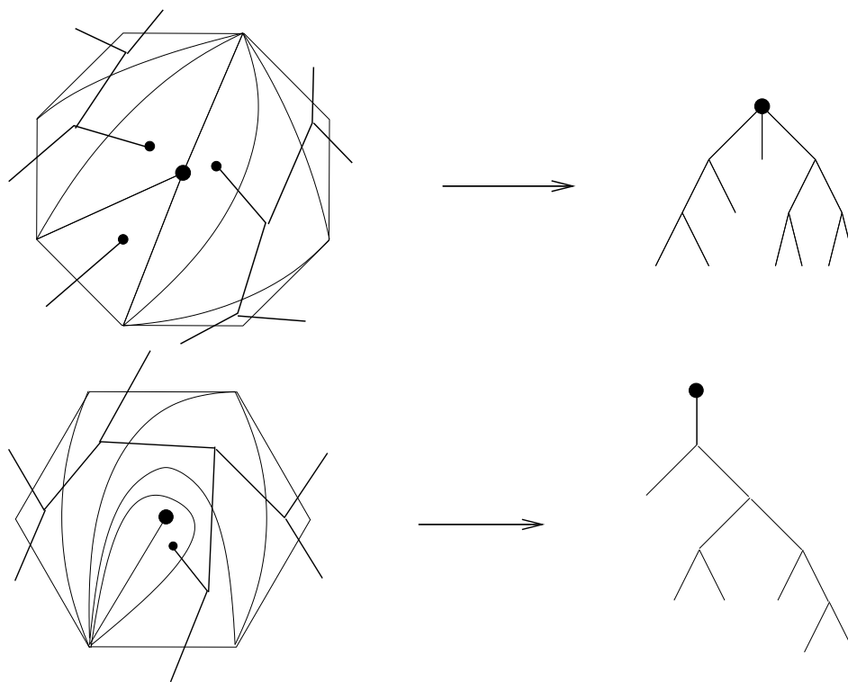
Figure 13: Triangulation and corresponding tree.
