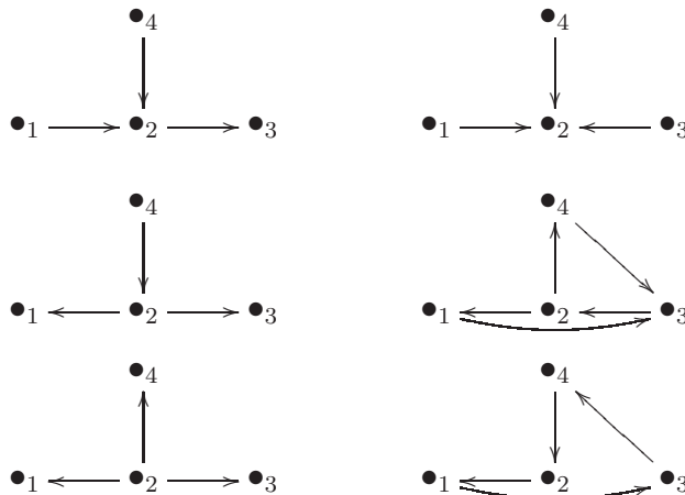
Figure 1: The mutation class of D_4 .
