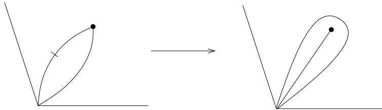
Figure 12: Drawing tagged edges as loops
