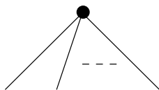
Figure 14: The tree R_n consisting of exactly n edges from the root.
