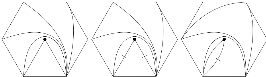
Figure 3: Examples of triangulations of the punctured 6-gon.
