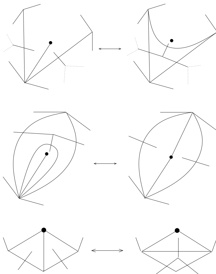
Figure 19: Mutation of triangulations and trees commutes. See proof of Proposition 8.1.
