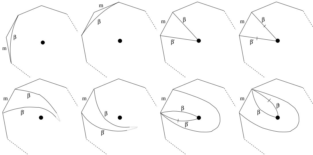
Figure 10: Extension at m .
