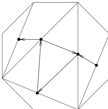
Figure 2: A triangulation \Delta of the regular 8-gon and the corresponding quiver \gamma_5(\Delta) of type A_5 .
