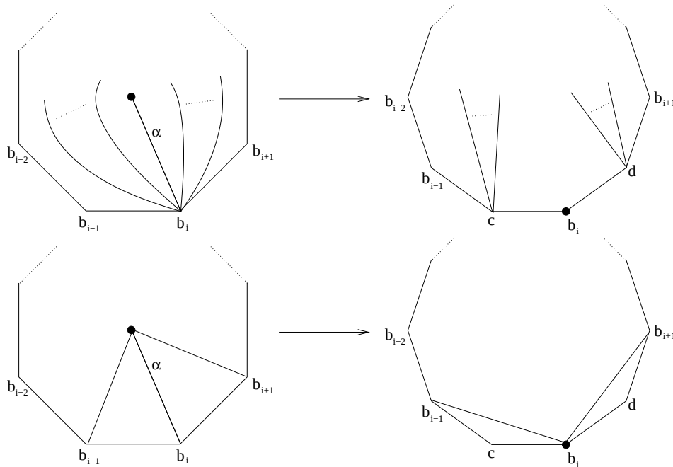
Figure 9: Factoring out a diagonal from the puncture to the border.
