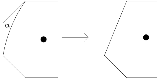
Figure 7: See the proof of Lemma 5.2
