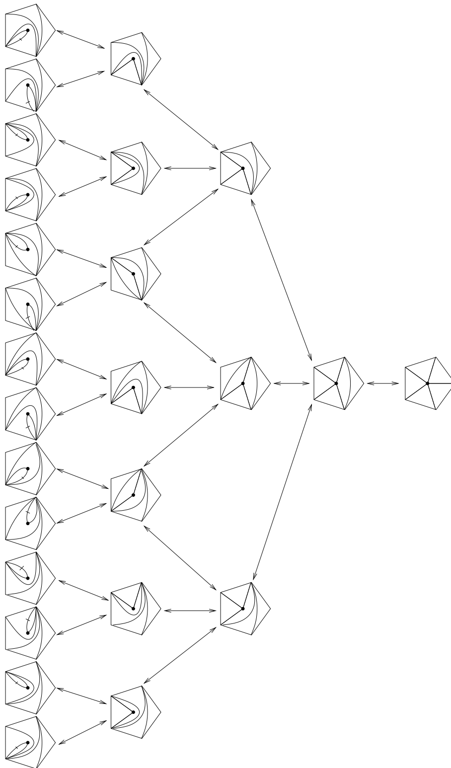
Figure 20: All triangulations of type D_5 .
