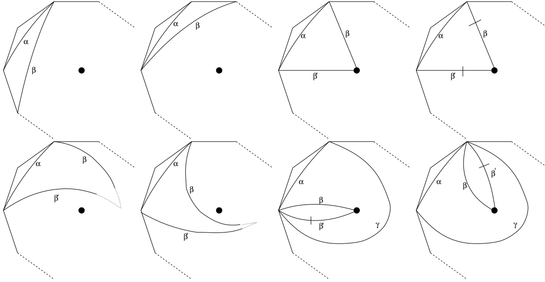
Figure 7: See the proof of Lemma 5.2
