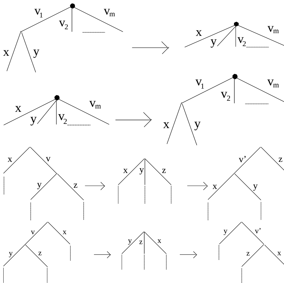
Figure 17: Mutation of a tree.
