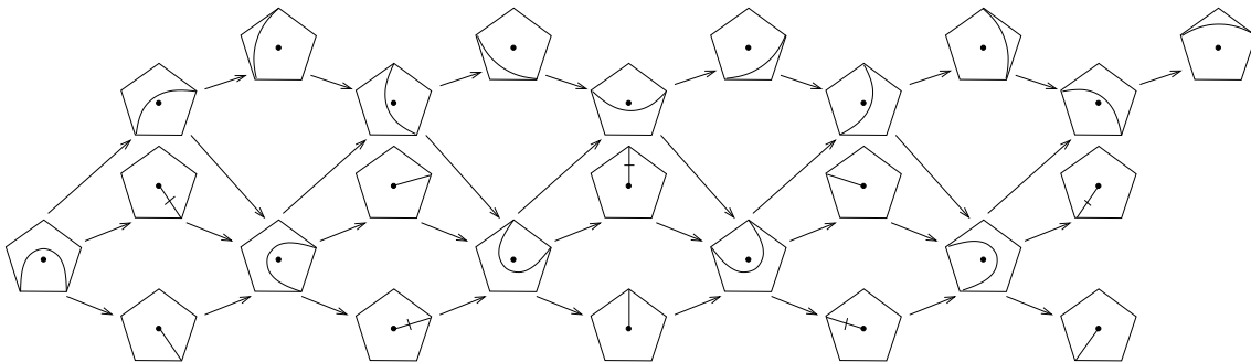
Figure 11: AR quiver for the cluster category in the D_5 case.
