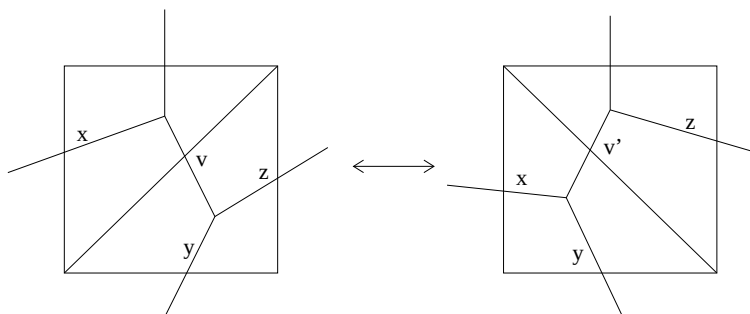
Figure 18: Mutation of triangulations and trees commute. See proof of Proposition 8.1.
