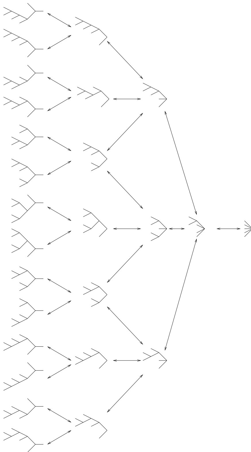
Figure 21: All trees of type D_5 .
