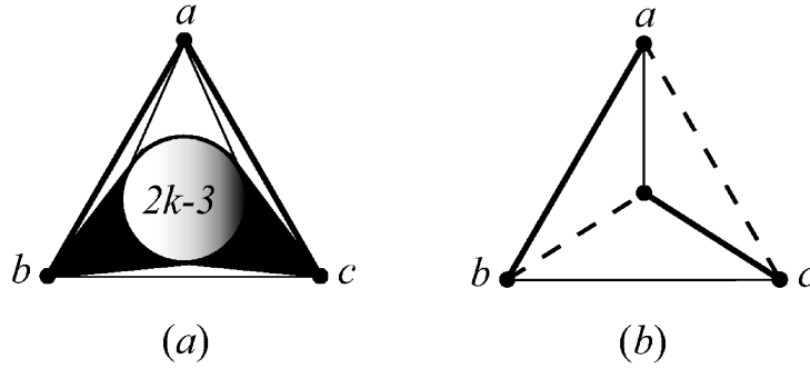
Figure 2: (\binom{2k-3}{2} + 2 \text{ or } +3) -Colorings without rainbow k -matchings.
