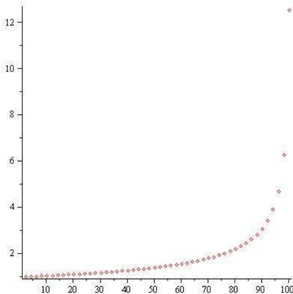
Figure 1: \mathbb{E}_e^{(100)} Y_k for k = 2, 4, \dots, 100 .
