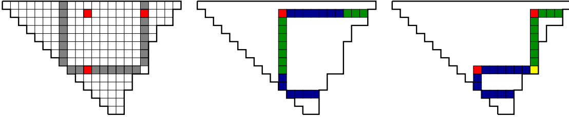
Figure 16: The punctured hook of a square is the disjoint union of the punctured hooks of projections onto shaded row and column. The yellow square is in the punctured hook of both projections.
