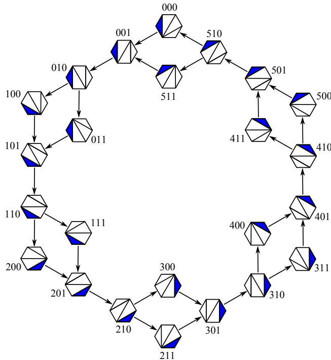
Figure 2: \Gamma_6 with orientation
