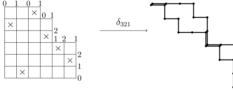
Figure 6: An example of the bijection \delta_{321} . The sequence j_0 \dots j_{2n} is written along the border of F .
