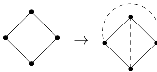
Figure 1: An extension of the smallest plane quadrangulation.
