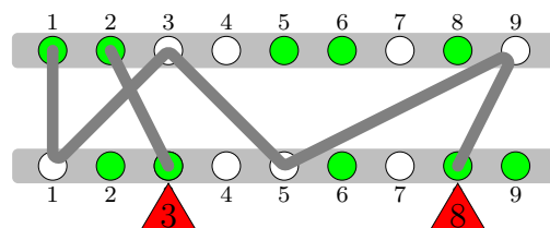
Figure 8: Bicoloured paths (drawn here as thick gray lines) starting in lower vertices 3 and 8 (see the running example in Figure 7).
