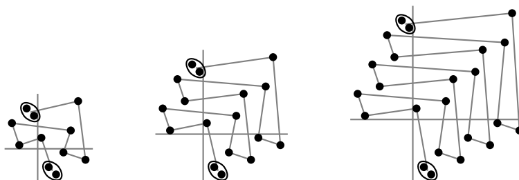
Figure 8: The first three elements of an infinite antichain in \text{Grid} \left( \begin{smallmatrix} \oplus 21 & \text{Av}(21) \\ & \oplus 21 \end{smallmatrix} \right) .
