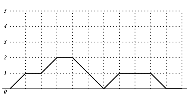
Figure 1: Example of a Motzkin path of size n = 11 .
