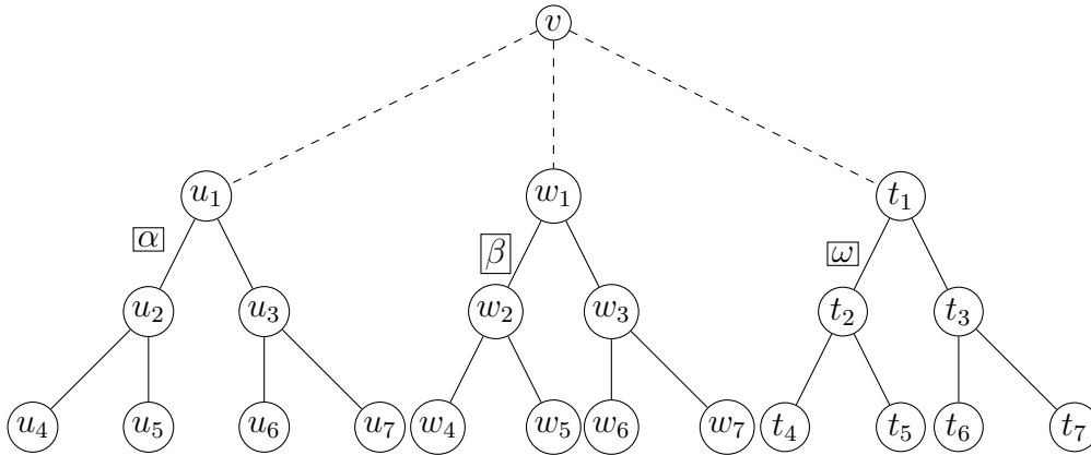
Figure 2: The precoloring
