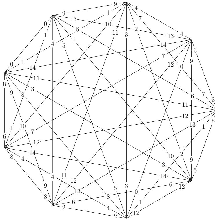
Figure 4: A 4-intersection edge-coloring of K_9 with 15 colors.
