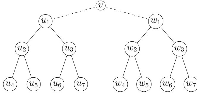
Figure 1: Example of vertex of degree 2
