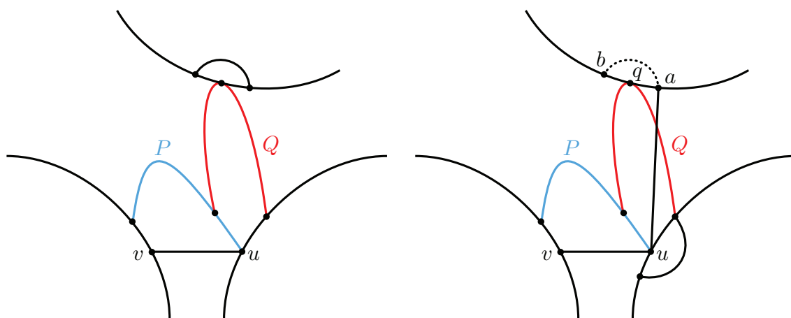
Figure 5: Two special cases for skip-and-glue fusions.
