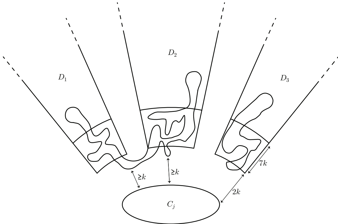
Figure 3: The subgraph F' .
