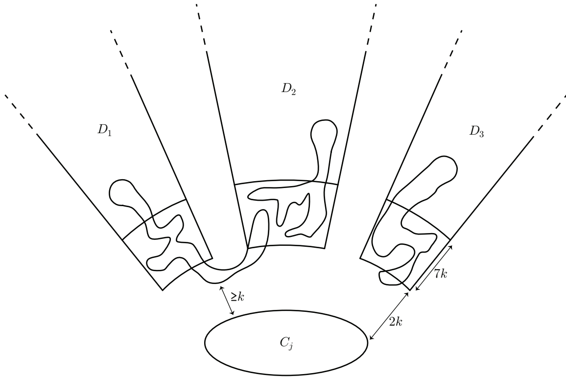
Figure 2: The subgraph F .
