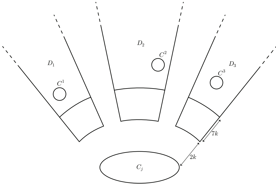
Figure 1: The cycle C_j with the cycles C^i .
