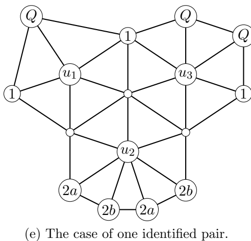
Figure 5: The case of Lemma 18.
