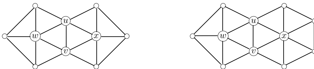
(a) Adjacent vertices u and v , with nonadjacent common 5-neighbors w and x .
