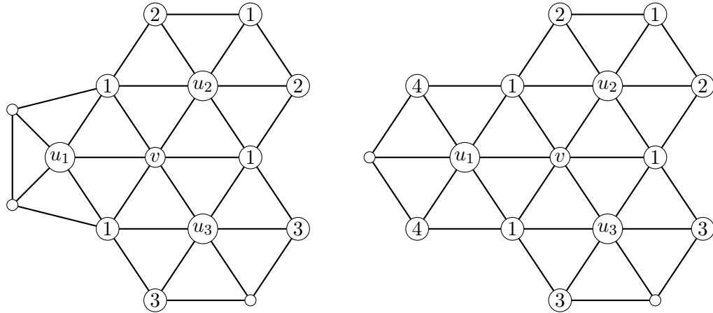
(a) A 6-vertex, v , with non-adjacent neighbors u_1, u_2 , and u_3 such that d(u_1) = 5 and d(u_2) = d(u_3) = 6 . (b) A 6-vertex, v , with non-adjacent 6-neighbors u_1, u_2 , and u_3 .
