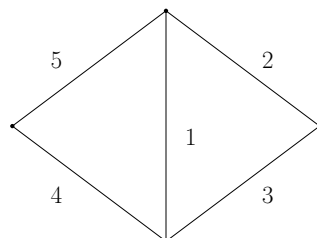
Figure 1: A graphic matroid.
