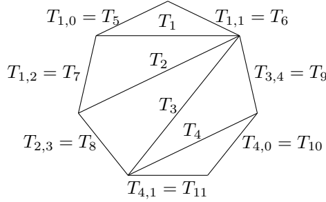
FIGURE 14. The initial triangulation of the quiver (Q, Q') in Example 2.1.
