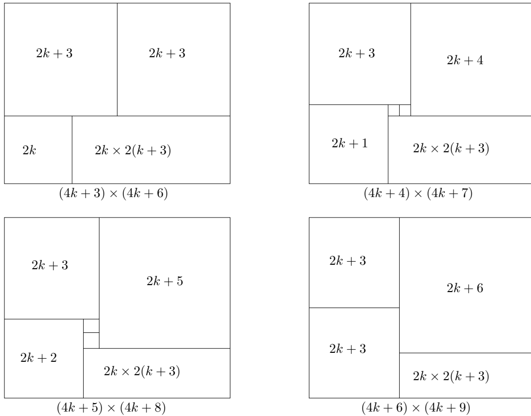
Figure 4: Dissecting a rectangle of size n \times (n+3) (Figure 1. from [10])
