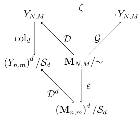
Figure 2: Rational Catalan maps in the non-coprime case.
