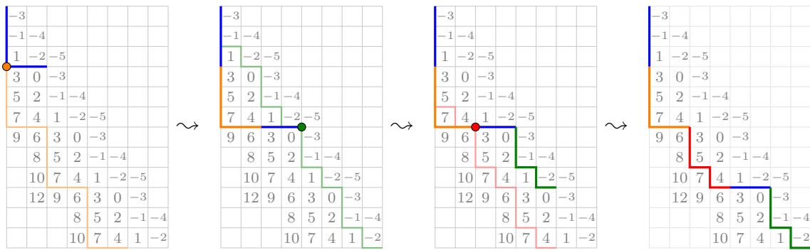
Figure 8: We apply the gluing algorithm to the periodic paths from Figure 6, using the graph from Figure 5. On each step we indicate the gluing point: the first intersection of the Dyck path built so far with the next periodic path.
