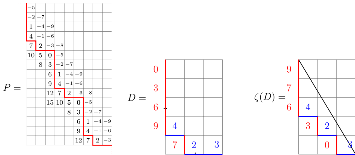
Figure 3: Here n = 5 and m = 3 . On the left is (a fragment of) the periodic path P = P(\{0, 3, 5, 6, 7, 8, \dots\}) , center is the diagram D = \mathcal{D}(\{0, 3, 5, 6, 7, 8, \dots\}) , and on the right is the diagram \zeta(D) .
