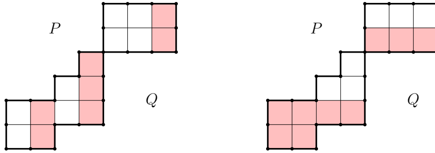
(a) \text{varea}(P, Q) = 2 + 3 + 2 = 7 (b) \text{vrarea}(P, Q) = 2 + 4 + 3 = 9
