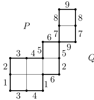
The bijection \Upsilon . Here \Upsilon(P, Q) = 341625978 \in \mathcal{S}_9(321) .
