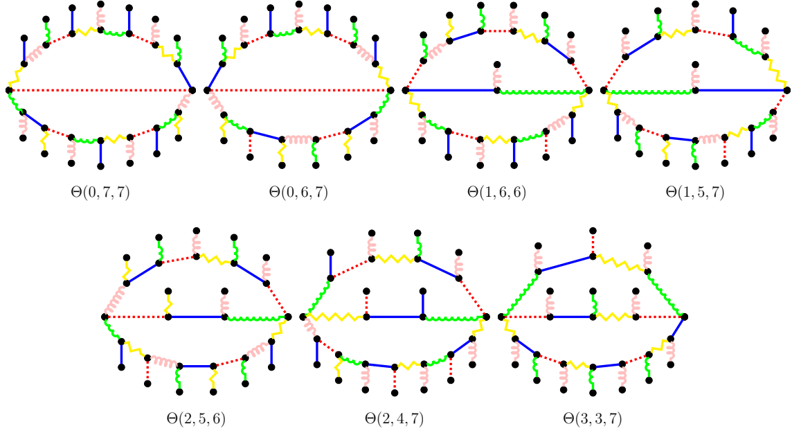
Figure 11: Strong edge-colorings of \Theta(t_1, t_2, t_3) . Style of line corresponds to color to make colors visible on a black and white print.
