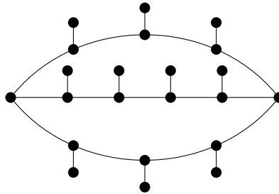
Figure 5: The graph G = \text{ex}_3(\Theta_{3,3,4}) with \text{mad}(G) = 2 + \frac{1}{6} and \chi'_s(G) = 6 .
