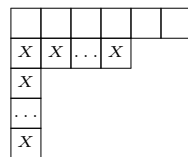
Figure 1a: \mu = (n) , with hook (m-s, 1^s) , 0 \leq s \leq m-2 , in row 2. The contribution to p_n p_m here is (-1)^s (n, m-s, 1^s) , if m \geq 2 .
