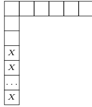
Figure 2b: \mu = (n - r, 1^r), 0 \leq r \leq n - 1 , with vertical strip of size m . The contribution to p_n p_m here is (-1)^{r+m-1}(n - r, 1^{r+m}), 0 \leq r \leq n - 1 .
