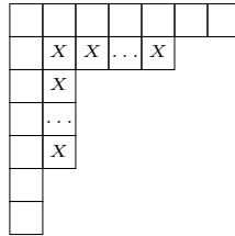
Figure 3: \mu = (n - r, 1^r), r \geq 1, n - r - 1 \geq 1 with attached hook (m - s, 1^s), 0 \leq s \leq m - 1 . The contribution to p_n p_m is (-1)^{r+s}(n - r, m - s + 1, 2^s, 1^{r-1-s}), 0 \leq s \leq m - 1, 1 \leq r \leq n - 2 .
