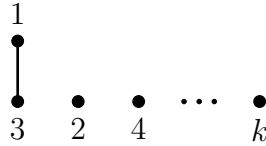
Figure 3: The POP in Theorem 5.
