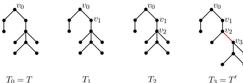
Figure 5: An illustration of the sequence transforming T into T' , where d = 3 and k = 10 . We also have s_0 = 2 , s_1 = 0 , and s_2 = 1 .
