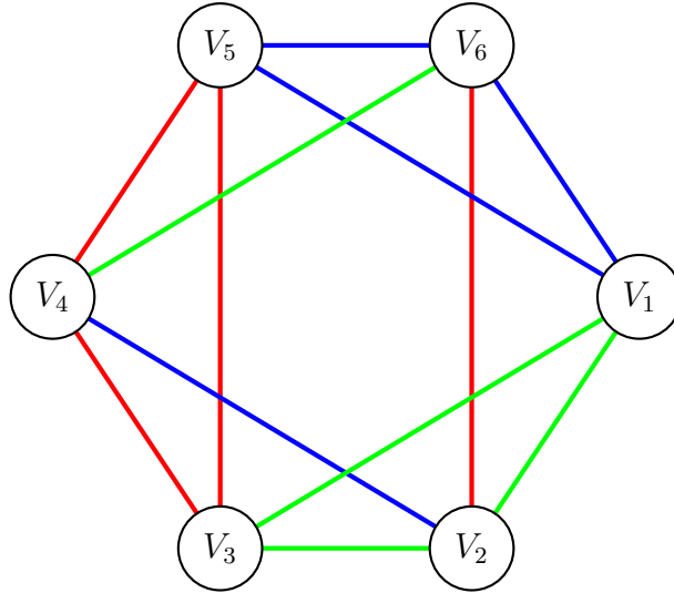
Figure 5: The limit graph of G for for all residue classes modulo 6.
