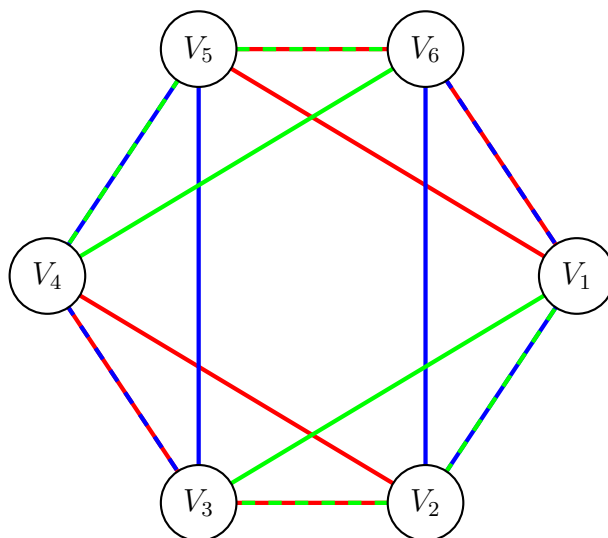
Figure 2: Optimal solutions of Linear Program 1 are subgraphs of this graph.
