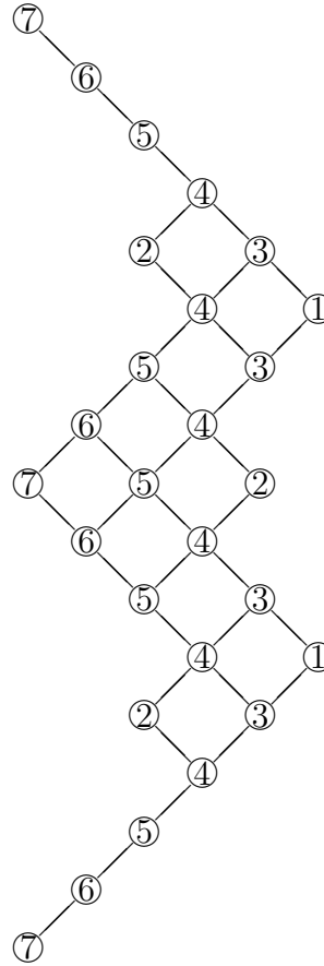
Figure 7: P_{E_7, \varpi_7}
