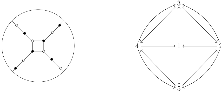
Figure 4.2: Left: on-shell diagram B' . Right: the associated quiver Q' .
