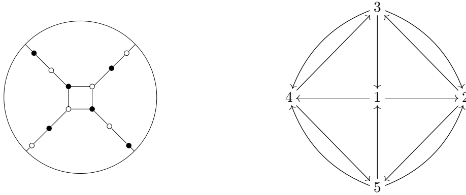
Figure 4.1: Left: on-shell diagram B . Right: the associated quiver Q .
