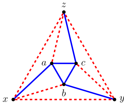
Figure 5: Mini-gadget (T, \pi)
